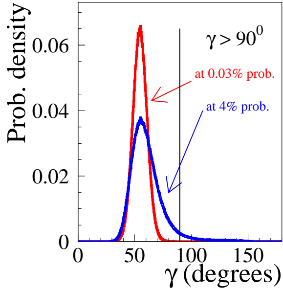
Figure 13: The p.d.f. for \gamma obtained with (red-clearer) and without (blue-darker) including the \Delta m_s constraint. The vertical line corresponds to \gamma = 90^\circ . The probabilities of \gamma > 90^\circ are also given.
