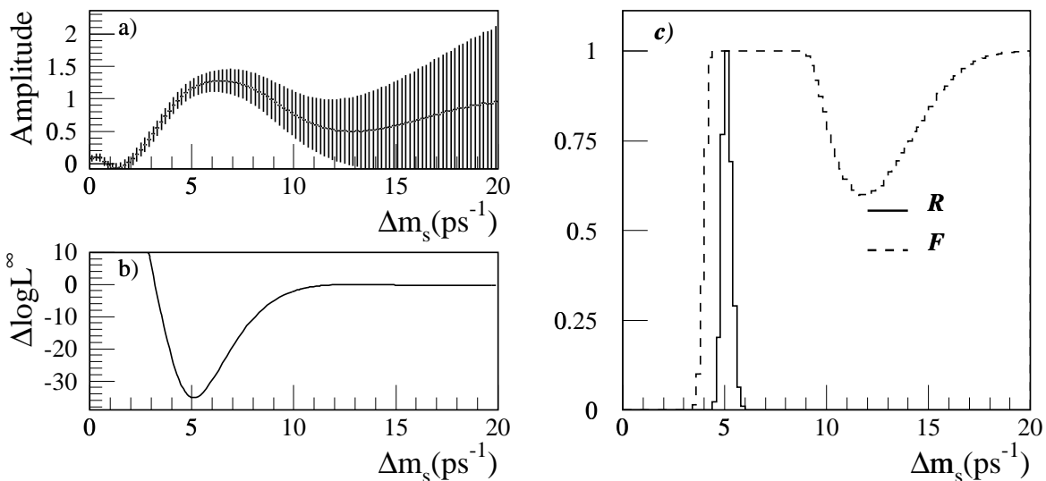
Figure 3: Amplitude analysis with \Delta m_s generated at 5 \text{ ps}^{-1} : a) amplitude spectrum, b) \Delta \log \mathcal{L}^\infty(\Delta m_s) , c) comparison between R and the function F used in the previous method. The maxima of the two functions have been rescaled to unity in order to ease the comparison
