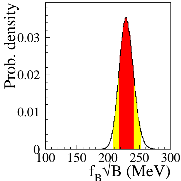
Figure 15: The p.d.f. for f_{B_d} \sqrt{\hat{B}_{B_d}} .
