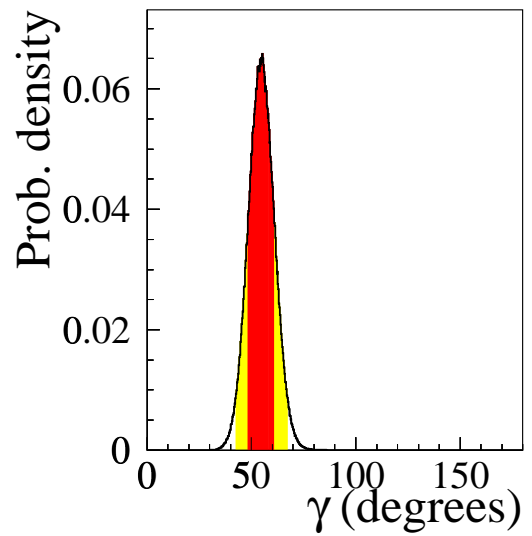
Figure 9: The p.d.f. for \sin(2\alpha) , \sin(2\beta) and \gamma . The red (darker) and the yellow (clearer) zones correspond respectively to 68% and 95% of the normalised area.
