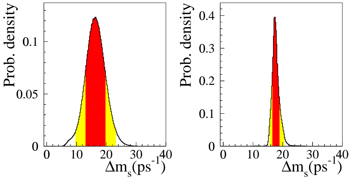
Figure 14: Probability distribution of \Delta m_s . The information from B_s^0 - \bar{B}_s^0 oscillations is used(not used) (distribution on the right(left)).
