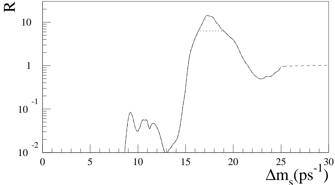
Figure 6: Comparison between different weight functions used in the fit. The curve determined by the continuous and dashed lines corresponds to the likelihood ratio obtained with, respectively, the measured amplitudes and the extrapolation to large values of \Delta m_s . The dotted curve is obtained by truncating the previous distribution once the amplitude becomes larger than one.
