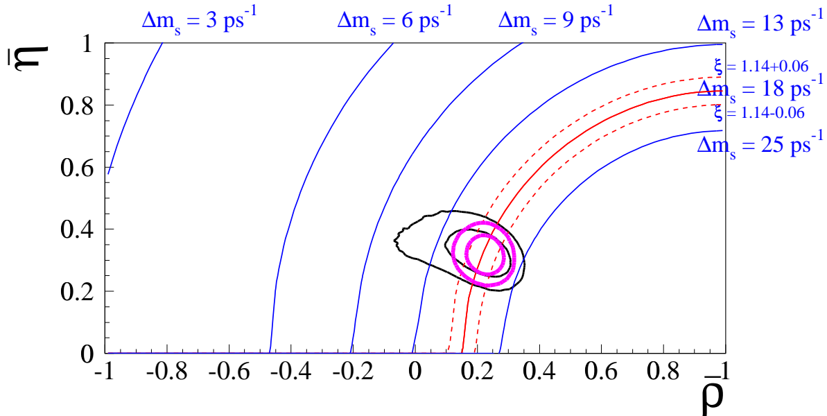
Figure 12: The allowed regions for \bar{\rho} and \bar{\eta} using the constraints given by the measurements of |\varepsilon_K| , |V_{ub}|/|V_{cb}| and \Delta m_d at 68% and 95% probability are shown by the thin contour lines. Selected regions for \bar{\rho} and \bar{\eta} when the constraint due to \Delta m_s is included have been superimposed using thick lines. The different continuous circles correspond to fixed values of \Delta m_s . Dashed circles, drawn on each side of the curve corresponding to \Delta m_s = 18.0 \text{ ps}^{-1} , indicate the effect of a variation by \pm 0.06 on \xi .
