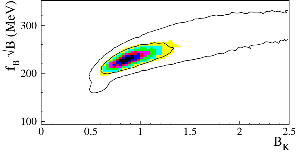
Figure 16: The 68% and 95% contours in the (f_{B_d}\sqrt{\hat{B}_{B_d}}, \hat{B}_K) plane.
