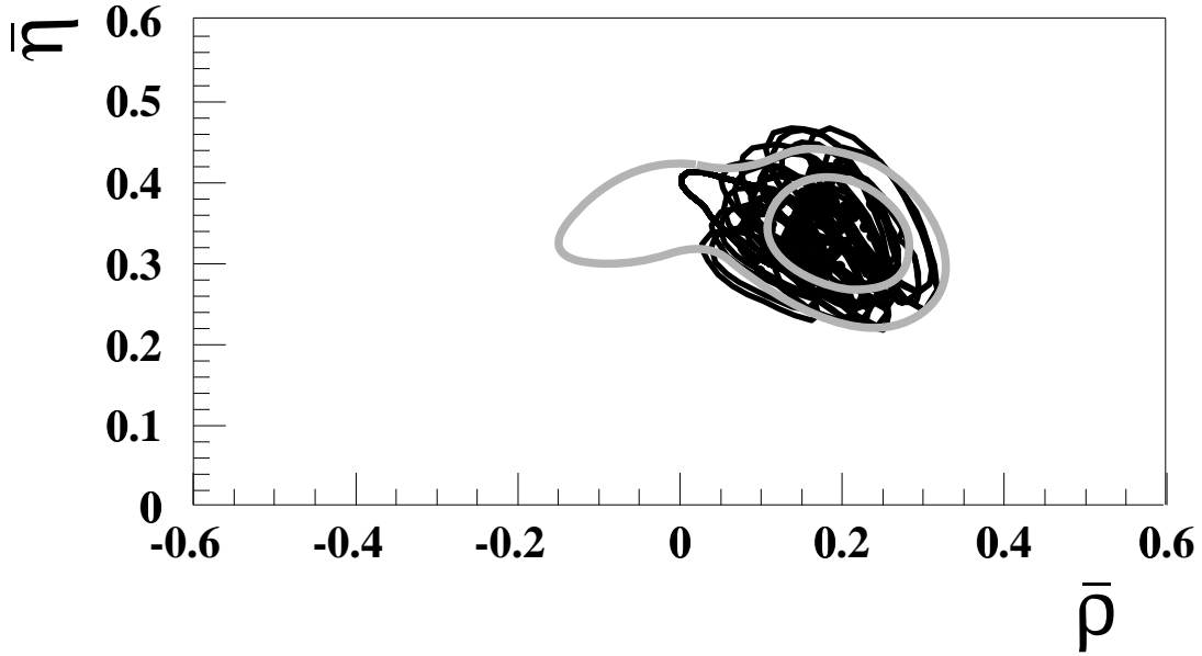
Figure 17: The contour corresponding to 95% probability in the standard approach, given by the internal continuous line, has been compared with the region spanned by 95% C.L. ellipses obtained in the 95% C.L. scanning method. The internal contour, corresponding to 68% probability in the standard approach, is also drawn.
