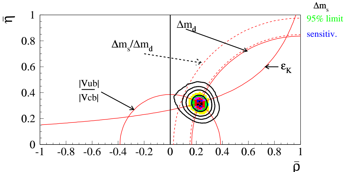
Figure 7: Allowed regions for \bar{\rho} and \bar{\eta} using the parameters listed in Table 2. The contours at 68%, 95%, 99% and 99.9% probability are shown. The full lines correspond to the central values of the constraints given by the measurements of |V_{ub}|/|V_{cb}| , |\epsilon_K| and \Delta m_d . The two dotted curves correspond, from left to right respectively, to the 95% upper limit and to the value of the sensitivity obtained from the experimental study of B_s^0 - \bar{B}_s^0 oscillations.
