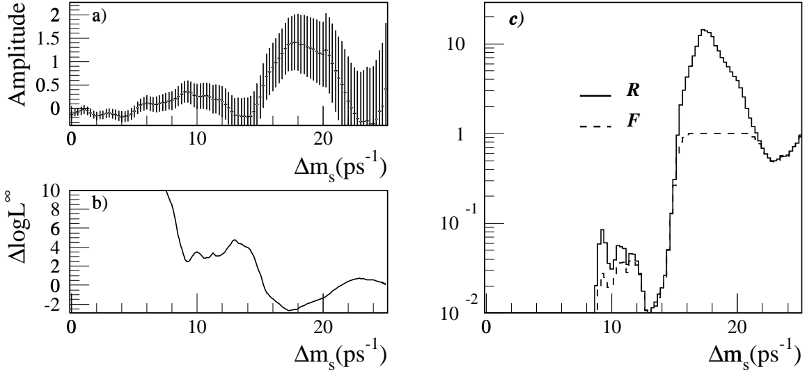
Figure 4: World average amplitude analysis: a) amplitude spectrum, b) \Delta \log \mathcal{L}^\infty(\Delta m_s) , c) comparison between R and the function used in the previous method.
