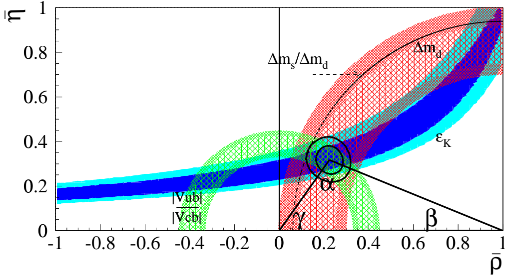
Figure 8: The allowed regions for \bar{\rho} and \bar{\eta} (contours at 68%, 95%) are compared with the uncertainty bands (at 68% and 95% probabilities) for |V_{ub}|/|V_{cb}| , |\epsilon_K| , \Delta m_d and the limit on \Delta m_s/\Delta m_d (dotted curve).
