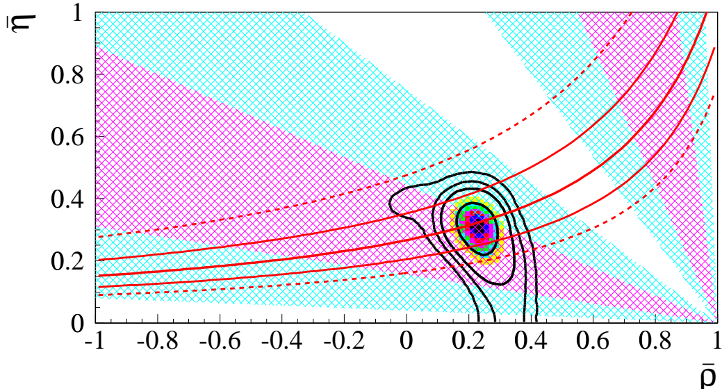
Figure 10: The allowed regions (at 68%, 95%, 99% and 99.9% probability) for \bar{\rho} and \bar{\eta} using the constraints given by the measurements of |V_{ub}|/|V_{cb}| , \Delta m_d and \Delta m_s . The constraint due to |\varepsilon_K| is not included. The regions (at 68% and 95% probability) selected by the measurements of |\varepsilon_K| (continuous ( 1\sigma ) and dotted ( 2\sigma ) curves) and \sin(2\beta) (darker ( 1\sigma ) and clearer ( 2\sigma ) zones) are shown. For \sin(2\beta) the two solutions are displayed.
