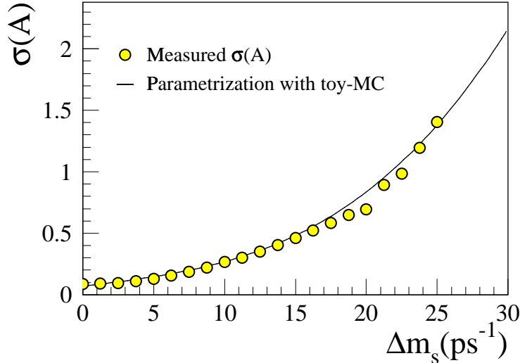
Figure 5: Comparison between the error distribution computed with a toy-MC (solid line) and the measured amplitude errors (circles).
