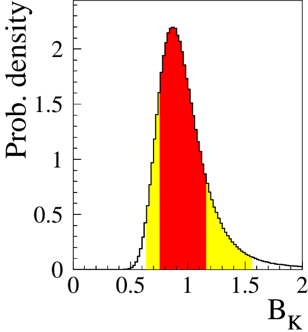
Figure 11: The p.d.f. for \hat{B}_K^{\text{b-phys}} .
