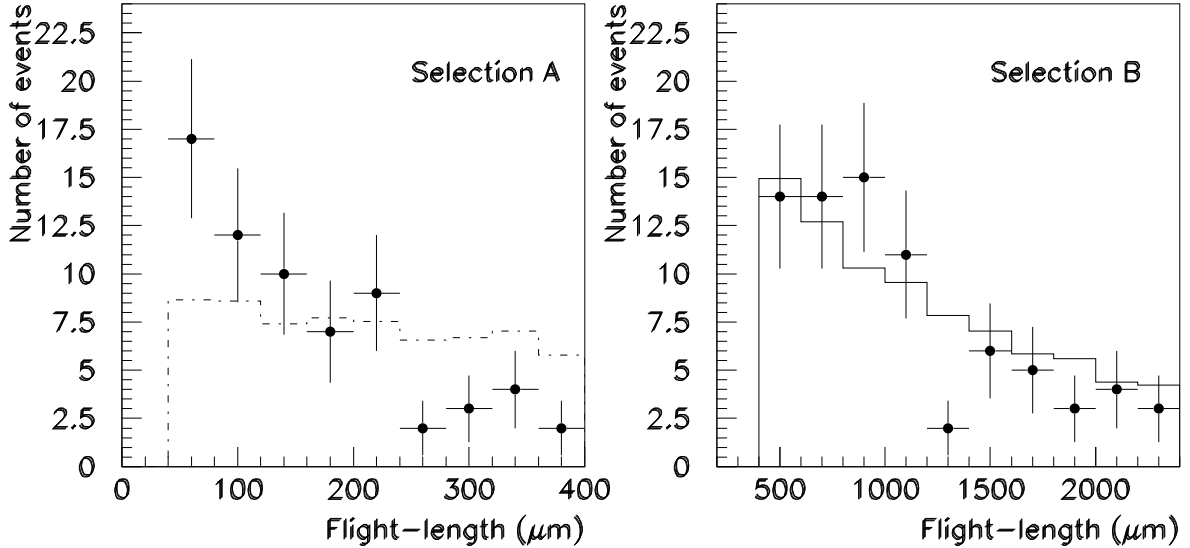
Figure 3: Flight-length distributions of charged charm candidates decaying into three particles. The histograms represent the flight-length distributions given by the Monte Carlo simulation for D^+ and D_s^+ , normalised to the number of observed events.
