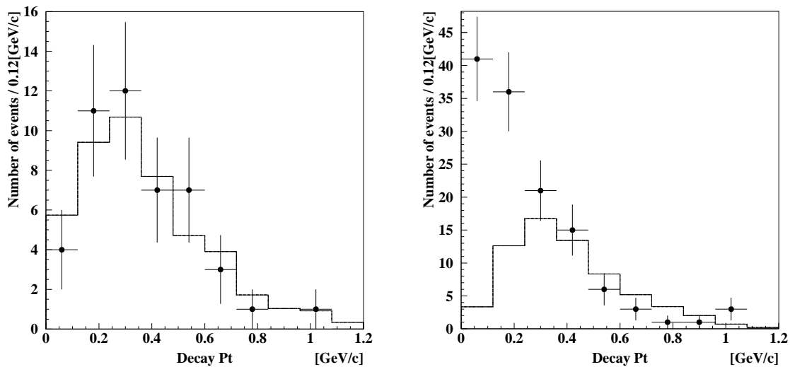
Figure 4: Decay p_T distribution for a subsample (about 70%) of events from selection A (left) and selection B (right) C1 events. The histograms represent the distribution of charged charm hadrons given by Monte Carlo simulation. Events with P_T > 240 MeV/c were used for normalisation.
