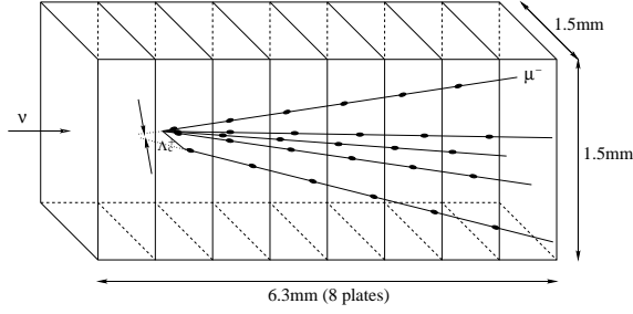
Figure 1: Schematic view of typical decays selected by criteria A. The ellipses represent the points measured by the UTS at each emulsion sheet interface.
