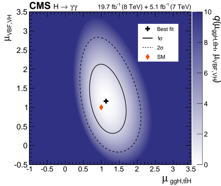
Figure 23: Map of the likelihood ratio q(\mu_{\text{ggH, ttH}}, \mu_{\text{VBF, VH}}) with m_H treated as an unconstrained parameter. The 1\sigma and 2\sigma uncertainty contours are shown. The cross indicates the best-fit values, (\hat{\mu}_{\text{ggH, ttH}}, \hat{\mu}_{\text{VBF, VH}}) = (1.13, 1.16) , and the diamond represents the SM expectation.
