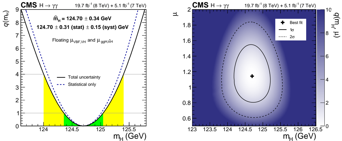
Figure 22: (left) Scan of the likelihood ratio, q , as a function of the hypothesised mass when \mu_{ggH, t\bar{t}H} and \mu_{VBF, VH} are allowed to vary independently. (right) Map of q(m_H, \mu) showing the 1 \sigma and 2 \sigma regions, and the best-fit point (\hat{m}_H, \hat{\mu}) = (124.70 \text{ GeV}, 1.14) .
