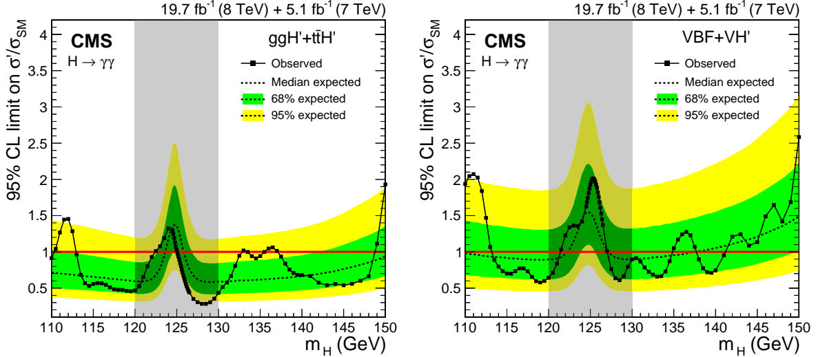
Figure 28: Exclusion limits on \sigma' / \sigma_{\text{SM}} for a second Higgs-boson-like state produced with gluon-gluon fusion only (left) or VBF and VH only (right) taking the observed state at 125 GeV as part of the background. The shading indicates a window with a width of 10 GeV, centred at the best-fit mass, where the expected sensitivity to a second Higgs boson is severely degraded due to the presence of the already observed state.
