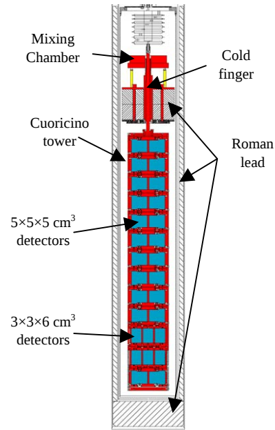
Fig. 1. Scheme of the Cuoricino tower inside the dilution refrigerator.
