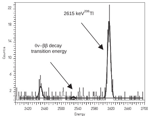
Fig. 3. Total background spectrum (in anticoincidence between the detectors) in the region of neutrinoless DBD of ^{130}\text{Te} . The solid curves represent the best fit (lowest) and the 68% and 90% CL excluded signals.
