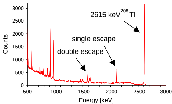
Fig. 2. Sum spectrum of all the 5 \times 5 \times 5 \text{ cm}^3 crystal obtained during a ^{232}\text{Th} calibration.
