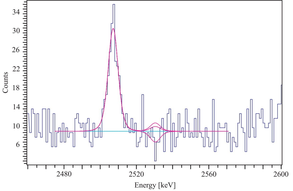
Figure 2: CUORICINO spectrum in the 0\nu\beta\beta region
