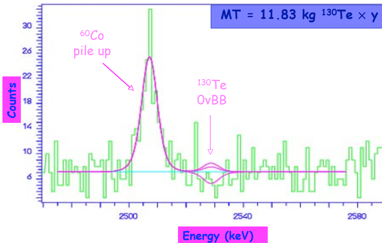
Background sum spectrum of all detectors in the DBD region
