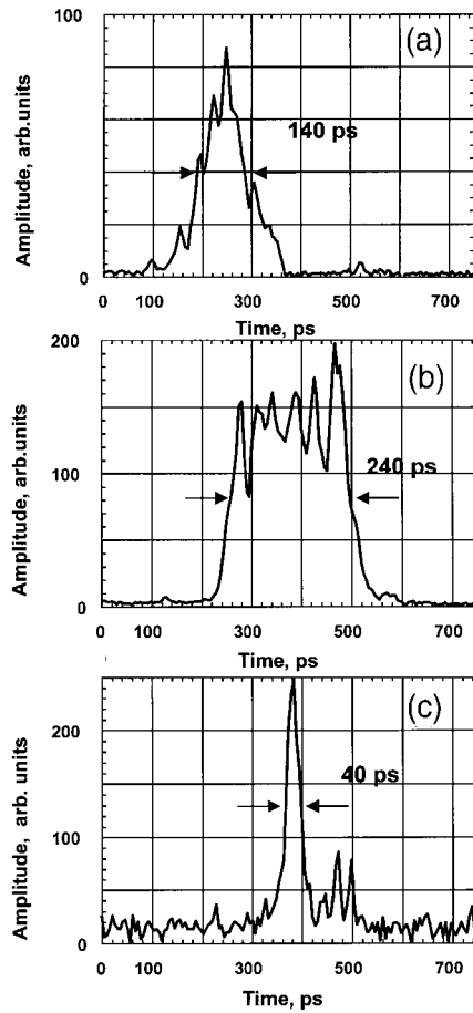
Figure 4.23: Temporal dynamics of the 10.6 \mu\text{m} CO 2 pulse at the Neptune Laboratory: (a) pulse injected in the amplifier, (b) pulse after the first pass of the amplifier, (c) pulse after three passes in the amplifier and after self-chirping into the plasma shutter.
