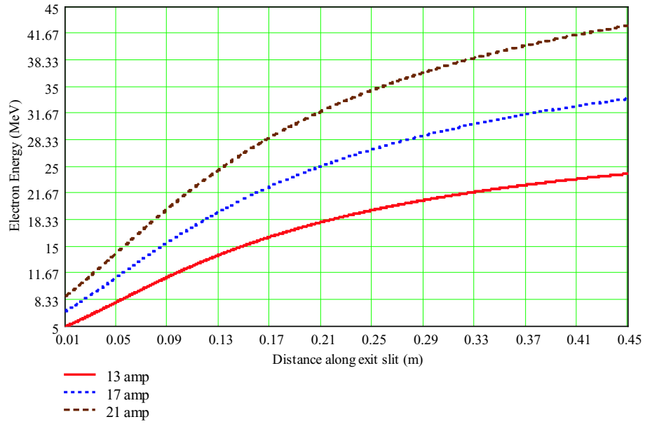
Figure 4.34: Calibration of final energy spectrometer.
