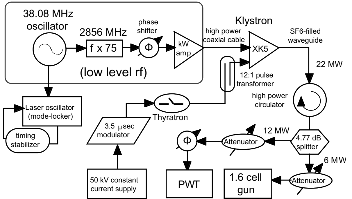
Figure 4.4: Schematic of Neptune radiofrequency system
