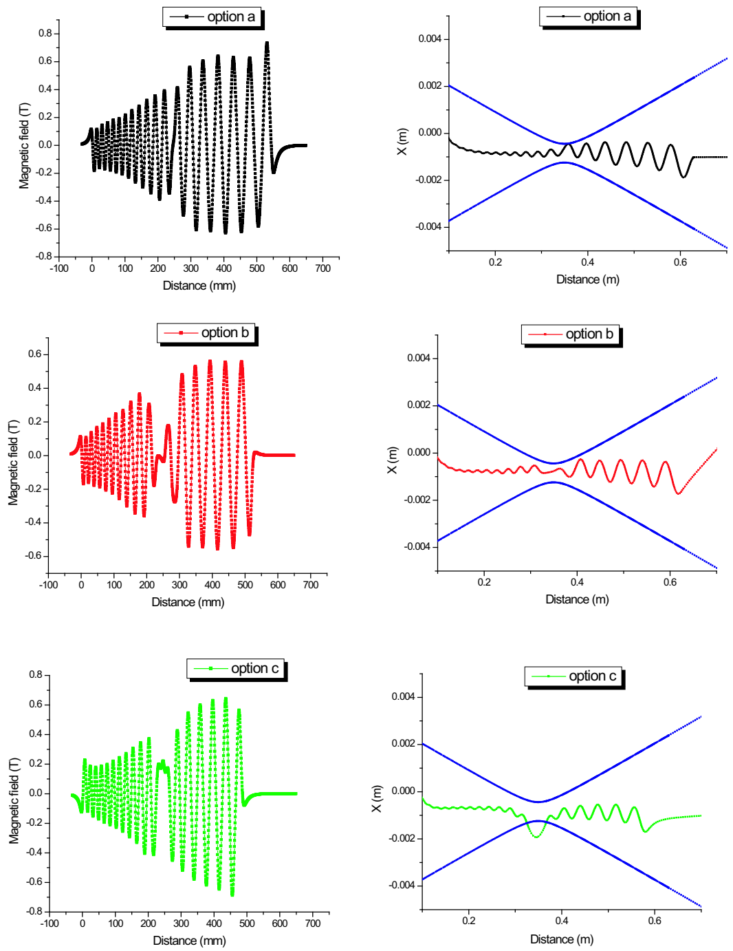
Figure 2.9: Magnetic field profile and electron trajectories for three different options to compensate a strong Guoy phase shift.
