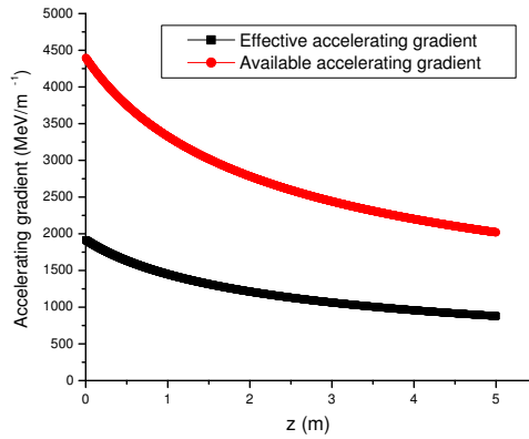
Figure 2.3: Constant K Inverse Free Electron Laser Accelerator. In 5 m the particles can be accelerated from 5 GeV to 10 GeV using a 10^{18} \text{ W/cm}^2 1.06 \mu\text{m} laser. When the period increases the magnetic field amplitude decreases to keep constant K . The energy is only growing as \sqrt{z} , but the radiation losses are controlled.
