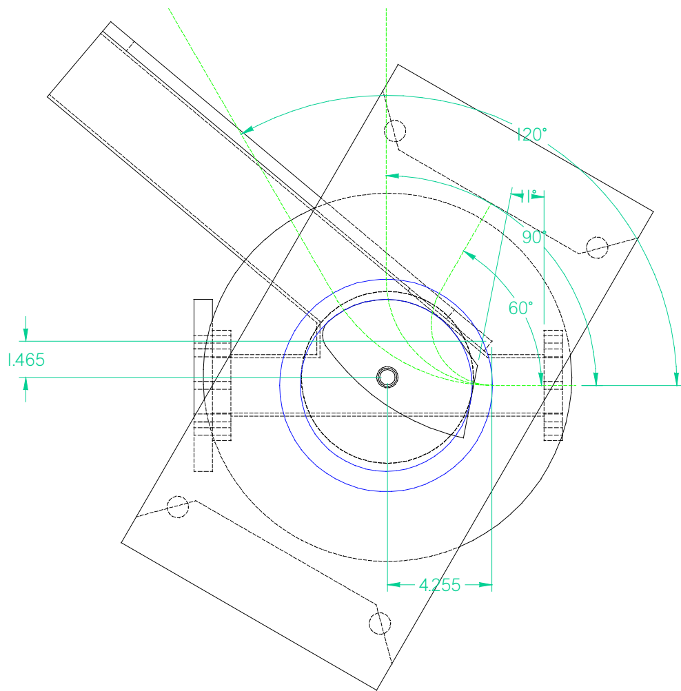
Figure 4.30: Trajectories inside the Browne-Buechner spectrometer.
