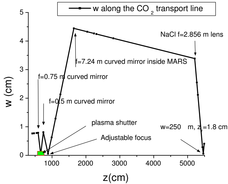
Figure 4.24: Spot size of CO 2 during transport to the bunker.
