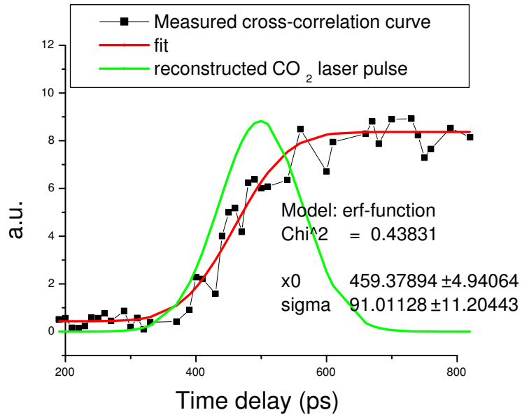
Figure 4.36: Typical electron beam/ CO 2 laser cross correlation curve.
