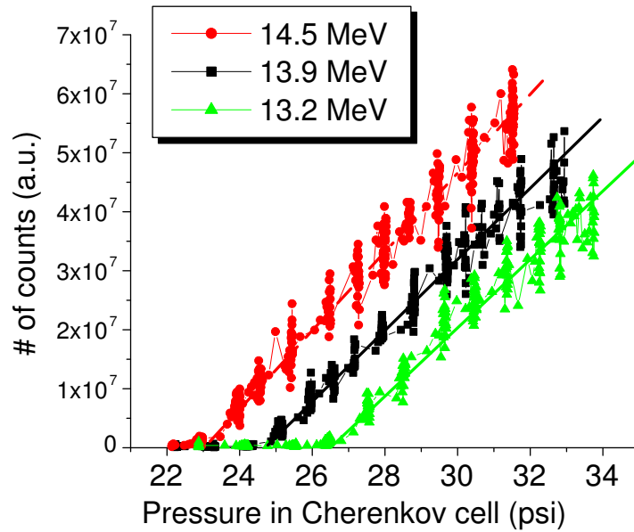
Figure 4.10: Results of the Cherenkov measurements for three different electron beam energy
