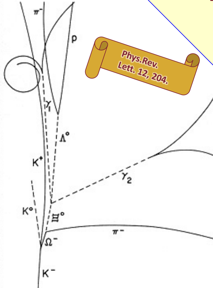
Brookhaven National Laboratory 80-inch hydrogen bubble chamber - 1964
