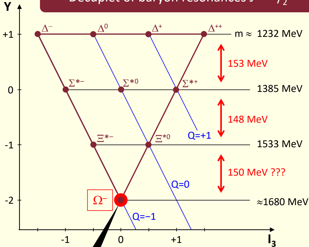
Decuplet of baryon resonances J^P = 3/2^+
