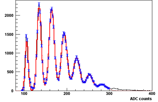
Fig. 1. ADC spectrum of the SiPM response to the low-intensity pulsed light fitted to a superposition of seven gaussian peaks.
