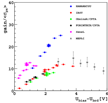
Fig. 3. The gain normalised to the corresponding values of pedestal width (top) and \langle \sigma_{px} \rangle (bottom) as functions of the overvoltage.
