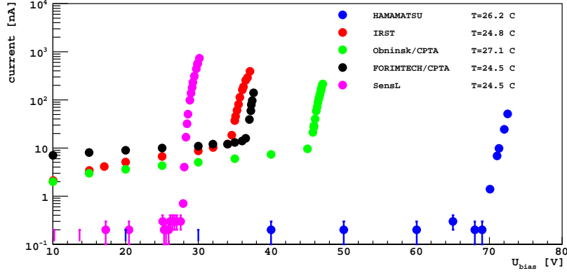
Fig. 2. – The current-voltage characteristics measured for the studied samples.
