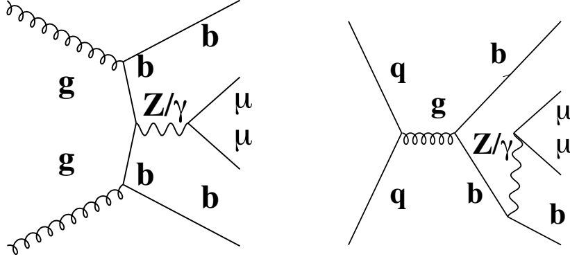
Figure 3: Typical diagrams contributing at “tree level” to the process gg \rightarrow Z/\gamma^* b\bar{b} \rightarrow \mu^+\mu^- b\bar{b} and q\bar{q} \rightarrow Z/\gamma^* b\bar{b} \rightarrow \mu^+\mu^- b\bar{b} .
