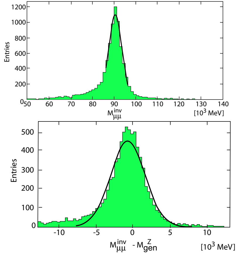
Figure 5: (top) Distribution of the invariant mass M_{\mu\mu}^{\text{inv}} reconstructed in b\bar{b}Z(\rightarrow \mu^+\mu^-) events. (bottom) Distribution of the difference between reconstructed and generated mass M_{\mu\mu}^{\text{inv}} - M_{\text{gen}}^Z for the same sample of events.
