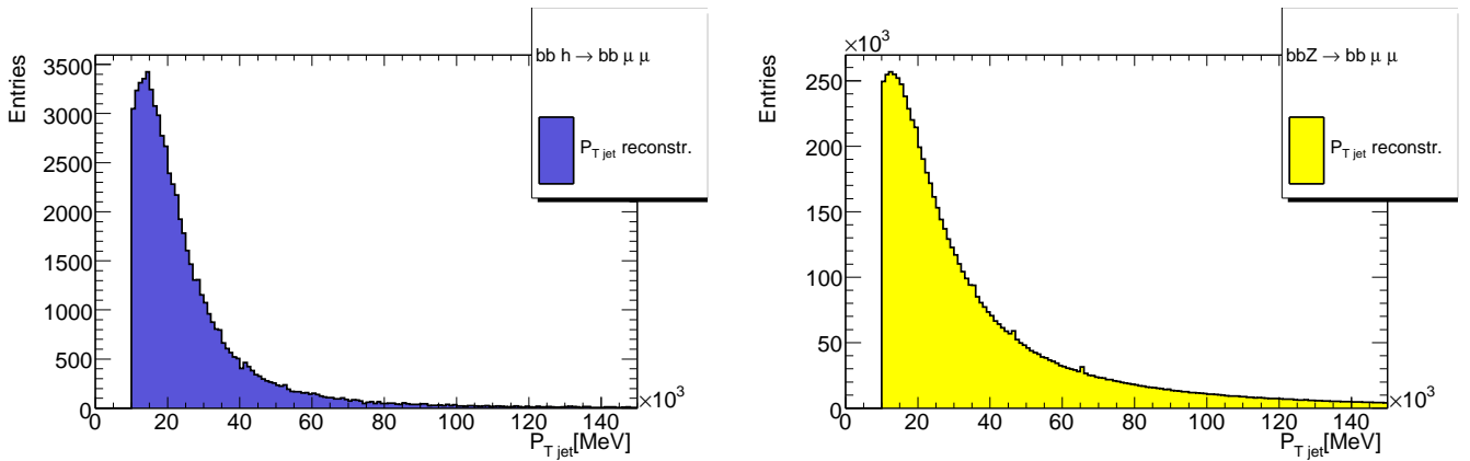
Figure 7: After 1-2 cuts. Distributions of the reconstructed jet transverse momentum P_{Tjet} are plotted after cuts 1 and 2 (Table 5) for : a) bbh \rightarrow bb\mu^+\mu^- events at the reference point ( \tan\beta = 45 , m_h = 110.00 GeV), (left, dark blue); b) bbZ \rightarrow bb\mu^+\mu^- events (right, yellow). All distributions are normalized at \int \mathcal{L} dt = 300 \text{ fb}^{-1} . Entries are per bin width of 10^3 MeV.
