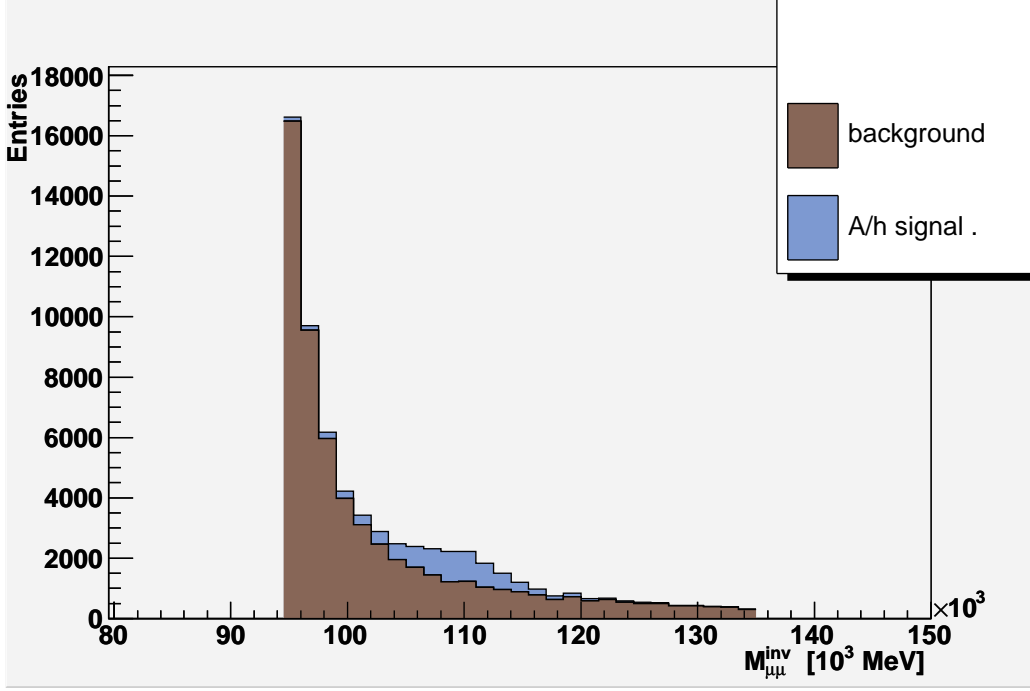
Figure 10: Distributions of the reconstructed \mu^+\mu^- invariant mass, M_{\mu\mu}^{\text{inv}} , for signal and background events, after the selection cuts 1-8 (Table 5) at the reference point ( \tan\beta = 45 , m_A = 110.31 GeV, m_h = 110.00 GeV). The two distributions are normalized at \int \mathcal{L} dt = 300 \text{ fb}^{-1} . The h/A signal (light blue) emerge over the background (Z, t\bar{t} and ZZ) (dark brown). Entries are per bin width of 1.5 \cdot 10^3 MeV.
