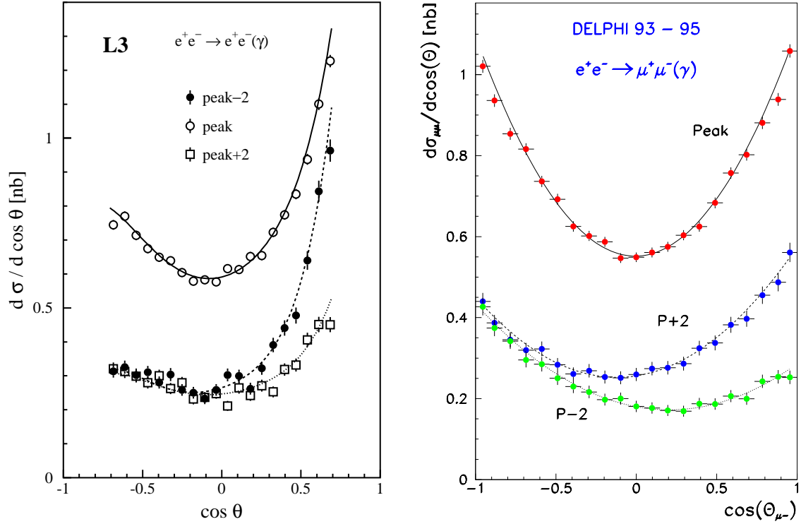
Figure 2.5: Distribution of the production polar angle, \cos \theta , for e^+e^- and \mu^+\mu^- events at the three principal energies during the years 1993–1995, measured in the L3 (left) and DELPHI (right) detectors, respectively. The curves show the SM prediction from ALIBABA [52] for e^+e^- and a fit to the data for \mu^+\mu^- assuming the parabolic form of the differential cross-section given in the text.
