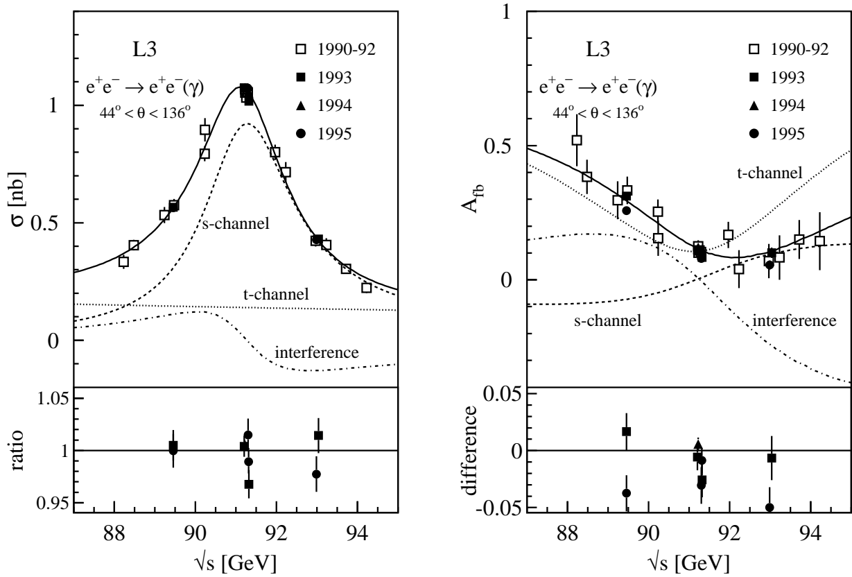
Figure 2.4: The energy dependence and the contributions from the s and t -channel diagrams and from the s - t interference for observables in the e^+e^- \rightarrow e^+e^-(\gamma) channel. Shown are the total cross-section (left) and the difference between the forward and backward cross-sections after normalisation to the total cross-section (right). The data points measured by the L3 collaboration refer to an angular acceptance of |\cos\theta| < 0.72 , an acollinearity \eta < 25^\circ and a minimum energy of E_{e^\pm} > 1 GeV. The lines represent the model-independent fit to all L3 data.
