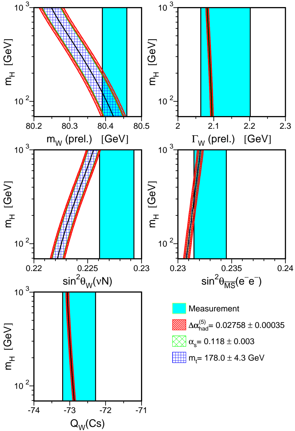
Figure 8.7: Comparison of the combined measurements of m_W and \Gamma_W , and the results from low Q^2 processes \sin^2 \theta_W(\nu N) , \sin^2 \theta_{\overline{MS}}(m_Z)(e^-e^-) and Q_W(\text{APV}) with the SM prediction as a function of the mass of the Higgs boson. The measurement with its uncertainty is shown as the vertical band. The width of the SM band arises due to the uncertainties in \Delta\alpha_{\text{had}}^{(5)}(m_Z^2) , \alpha_s(m_Z^2) and m_t in the ranges indicated. The total width of the band is the linear sum of these uncertainties. The direct measurements of m_W and \Gamma_W used here are preliminary.
