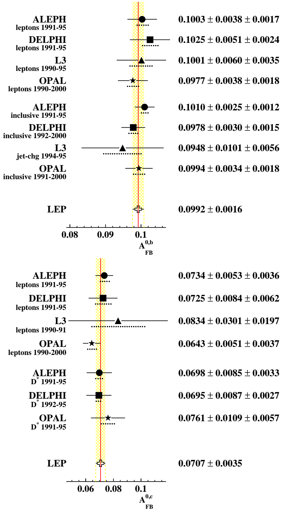
Figure 5.14: A_{\text{FB}}^{0,b} and A_{\text{FB}}^{0,c} measurements used in the heavy flavour combination, corrected for their dependence on parameters evaluated in the multi-parameter fit described in the text. The A_{\text{FB}}^{0,b} measurements with D-mesons do not contribute significantly to the average and are not shown in the plots. The experimental results are derived from the ones shown in Tables C.3 to C.8 combining the different centre of mass energies. The dotted lines indicate the size of the systematic error.
