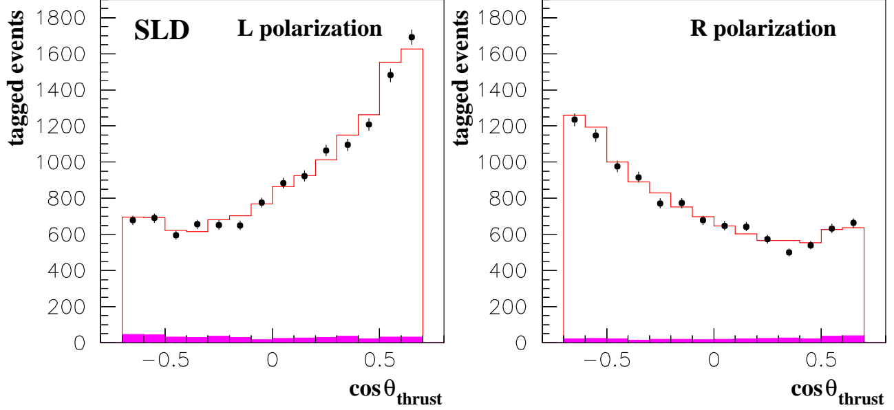
Figure 5.11: Reconstructed \cos\theta distributions from the SLD vertex charge \mathcal{A}_b analysis for events with left-handed and right-handed electron beam polarisations. The shaded region corresponds to udsc background in the sample estimated from Monte Carlo.
