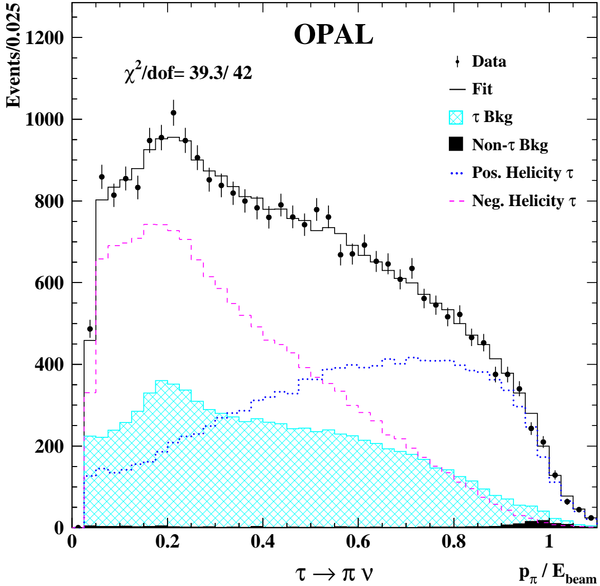
Figure 4.3: The measured distributions in the polarisation-sensitive variable for the \tau \rightarrow \pi \nu decays in the OPAL experiment. The variable is the ratio of the measured charged hadron momentum to the beam energy, which is an approximation of x_\pi = E_\pi/E_\tau . The data, shown by points with error bars, are integrated over the whole \cos \theta_{\tau^-} range. Overlaying this distribution are Monte Carlo distributions for the positive (dotted line) and negative (dashed line) helicity \tau leptons and for their sum including background, assuming a value for \langle \mathcal{P}_\tau \rangle equal to the fitted polarisation. The hatched histogram represents the Monte Carlo expectations of contributions from cross-contamination from other \tau decays and the dark shaded histogram the background from non- \tau sources. The level of agreement between the data and Monte Carlo distributions is quantified by quoting the \chi^2 and the number of degrees of freedom.
