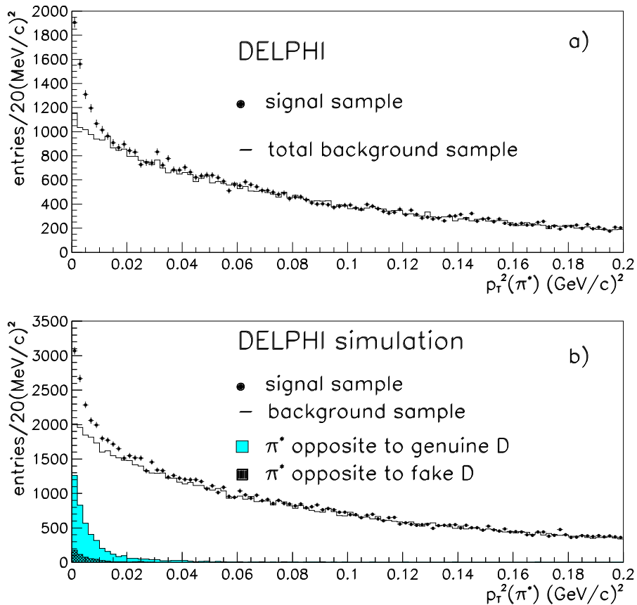
Figure 5.9: p_i^2 spectrum of the slow pion opposite a high energy D-meson candidate [132]. The points show pions with charge opposite that of the charm quark in the D-meson, while the histogram shows those with the same charge. The data is shown in a) and the simulation in b), with the signal component indicated separately.
