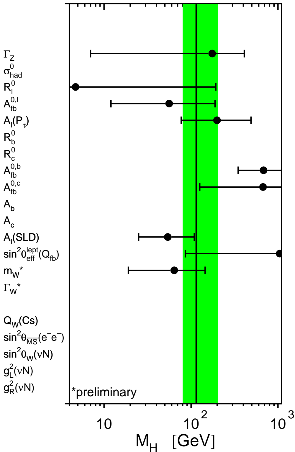
Figure 8.15: Constraints on the mass of the Higgs boson from each pseudo-observable. The Higgs-boson mass and its 68% CL uncertainty is obtained from a five-parameter SM fit to the observable, constraining \Delta\alpha_{\text{had}}^{(5)}(m_Z^2) = 0.02758 \pm 0.00035 , \alpha_S(m_Z^2) = 0.118 \pm 0.003 , m_Z = 91.1875 \pm 0.0021 GeV and Tevatron Run-I m_t = 178.0 \pm 4.3 GeV. Only significant constraints are shown. Because of these four common constraints the resulting Higgs-boson mass values cannot be combined. The shaded band denotes the overall constraint on the mass of the Higgs boson derived from all pseudo-observables reported in Table 8.3. The direct measurements of m_W and \Gamma_W used in that analysis are preliminary.
