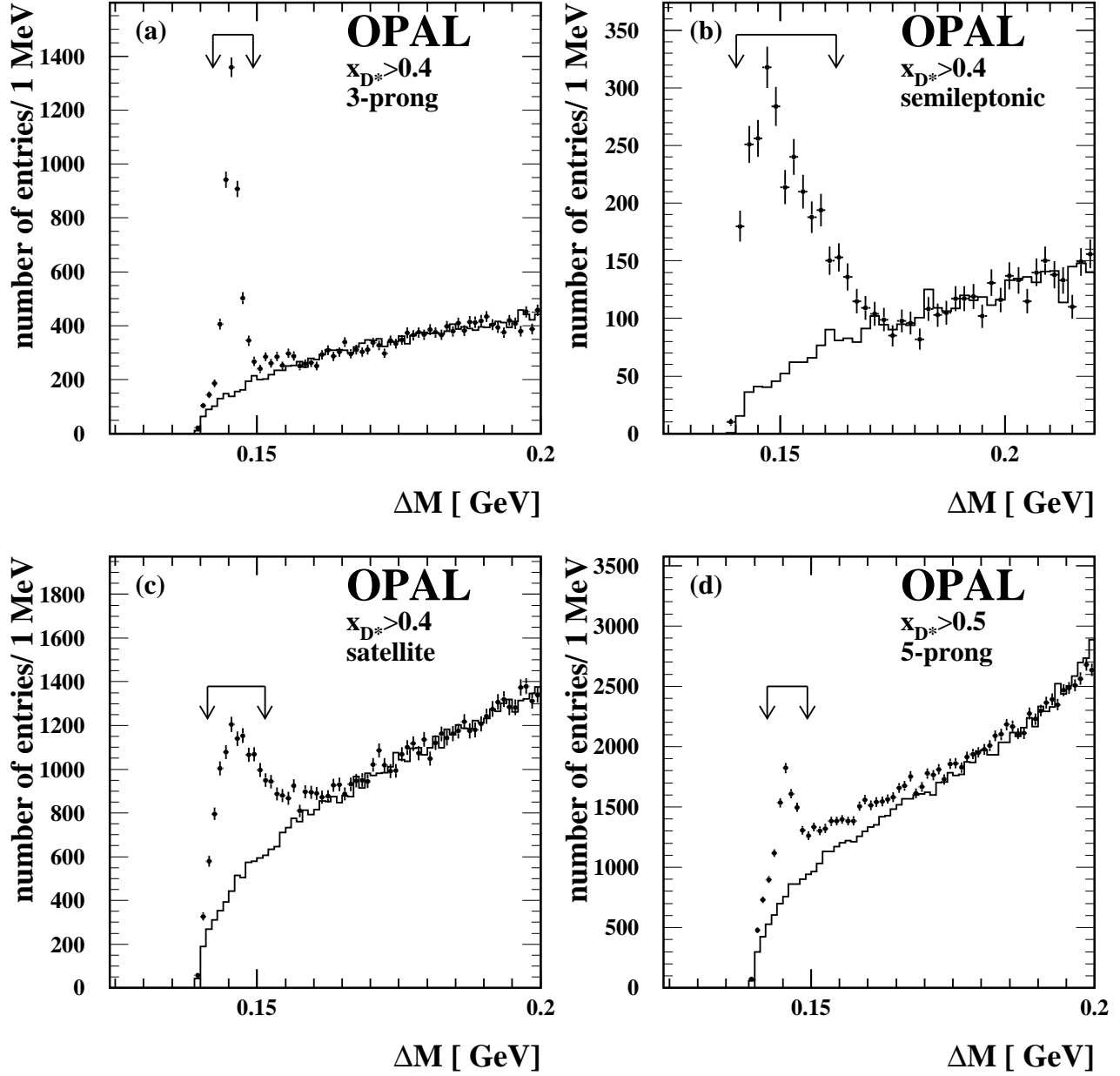
Figure 5.8: Mass difference spectrum m(\pi^+ D^0) - m(D^0) from OPAL in different channels [130]. In a) and d) the D^0 is fully reconstructed in the decay modes D^0 \rightarrow K^- \pi^+ and D^0 \rightarrow K^- \pi^+ \pi^+ \pi^- . In c) the decay mode D^0 \rightarrow K^- \pi^+ \pi^0 is used, where the \pi^0 is not reconstructed. This K^- \pi^+ mass peak is enhanced due to the large polarisation of the intermediate \rho^+ produced in the D^0 \rightarrow K^- \rho^+ \rightarrow K^- \pi^+ \pi^0 decay. In b) the D^0 is partially reconstructed in the semileptonic decay mode. The points with the error bars are the measured data. The solid histogram is the background estimated from measured data by a hemisphere mixing technique.
