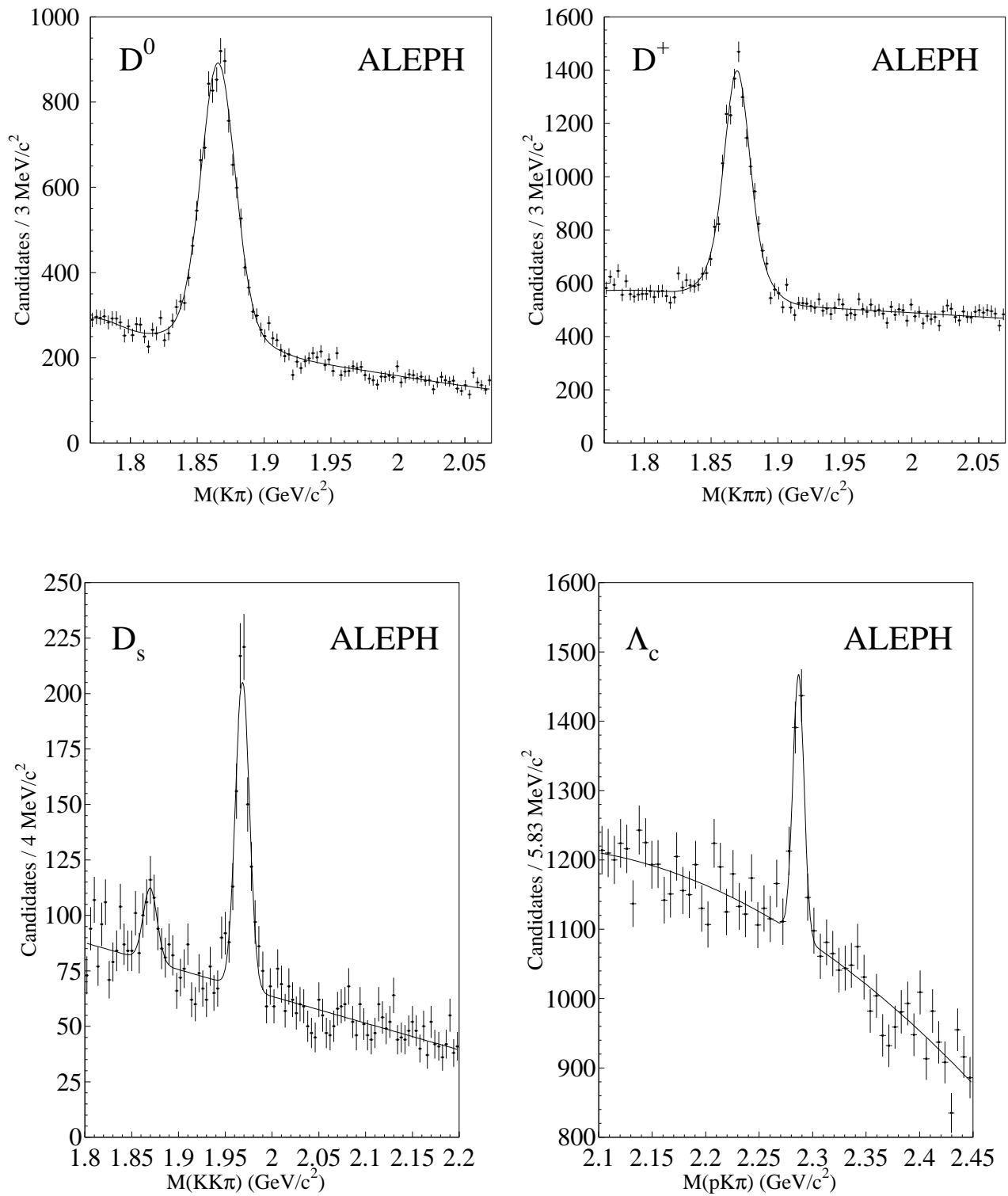
Figure 5.7: Mass spectra for D^0 \rightarrow K^- \pi^+ , D^+ \rightarrow K^- \pi^+ \pi^+ , D_s \rightarrow K^+ K^- \pi^+ and \Lambda_c^+ \rightarrow p K^- \pi^+ obtained by ALEPH [131].
