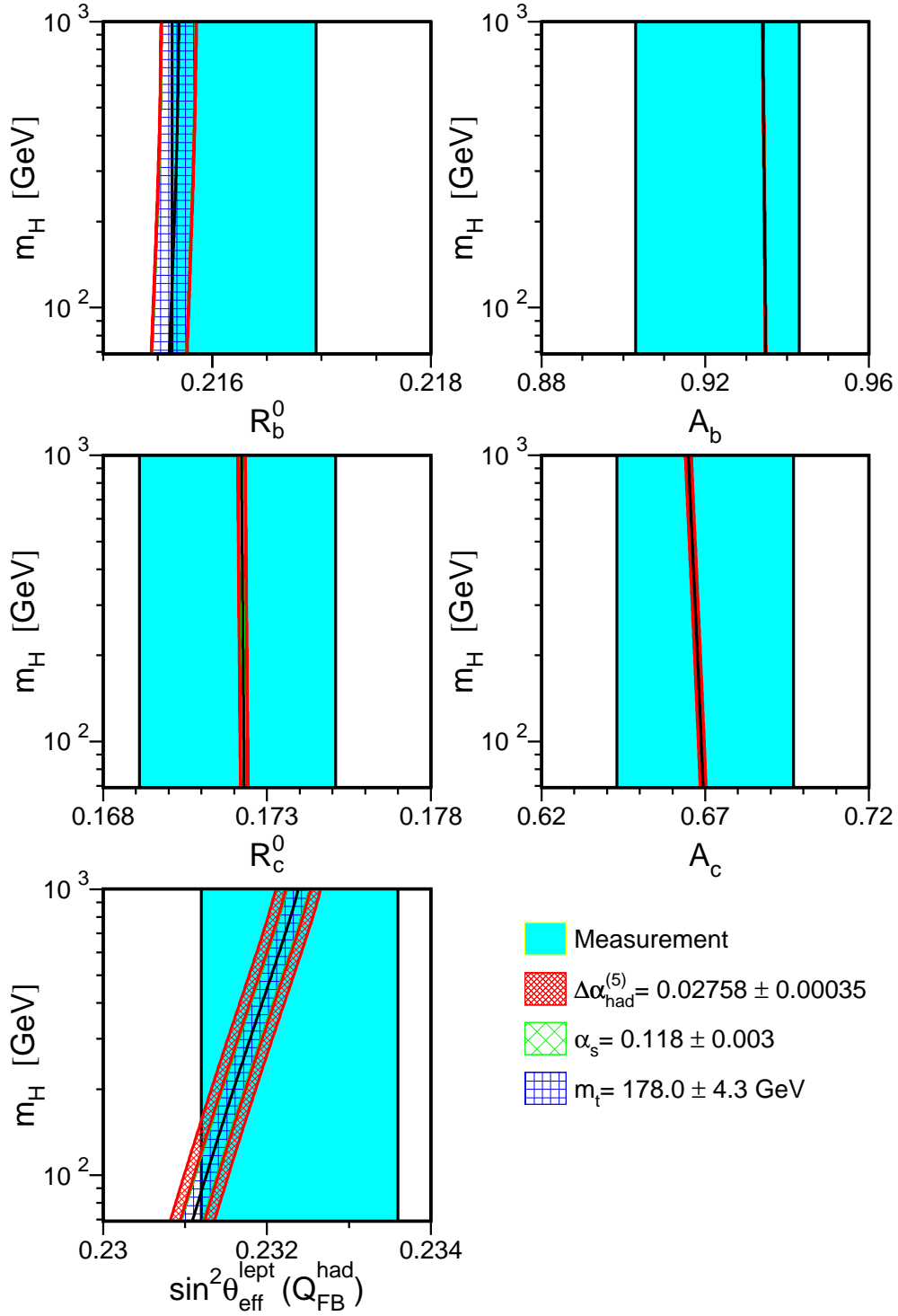
Figure 8.6: Comparison of the LEP/SLD combined measurements of R_b^0 , R_c^0 , \mathcal{A}_b , \mathcal{A}_c and \sin^2 \theta_{\text{eff}}^{\text{lept}}(Q_{\text{FB}}^{\text{had}}) with the SM prediction as a function of the mass of the Higgs boson. The measurement with its uncertainty is shown as the vertical band. The width of the SM band arises due to the uncertainties in \Delta\alpha_{\text{had}}^{(5)}(m_Z^2) , \alpha_s(m_Z^2) and m_t in the ranges indicated. The total width of the band is the linear sum of these uncertainties.
