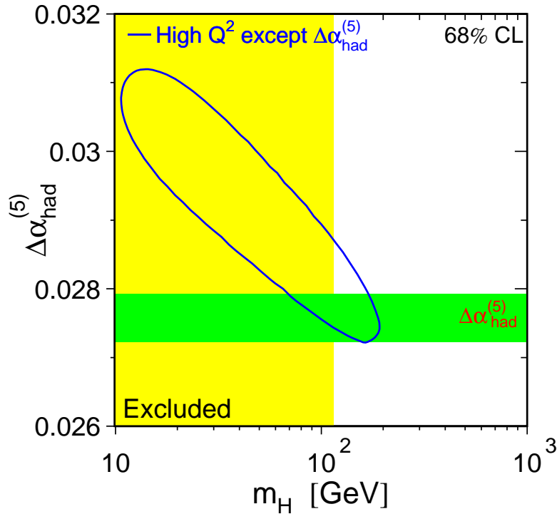
Figure 8.12: Contour curve of 68% probability in the (\Delta\alpha_{\text{had}}^{(5)}(m_Z^2), m_H) plane, based on all 18 measurements except the constraint on \Delta\alpha_{\text{had}}^{(5)}(m_Z^2) . The direct measurements of the excluded observable is shown as the horizontal bands of width \pm 1 standard deviation. The vertical band shows the 95% confidence level exclusion limit on m_H of 114.4 GeV derived from the direct search at LEP-II [39]. The direct measurements of m_W and \Gamma_W used here are preliminary.
