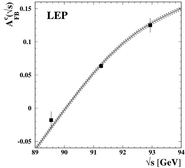
Figure 5.16: Energy dependence of A_{\text{FB}}^b and A_{\text{FB}}^c . The solid line represents the SM prediction for m_t = 178 GeV, m_H = 300 GeV, the upper (lower) dashed line is the prediction for m_H = 100 (1000) GeV.
