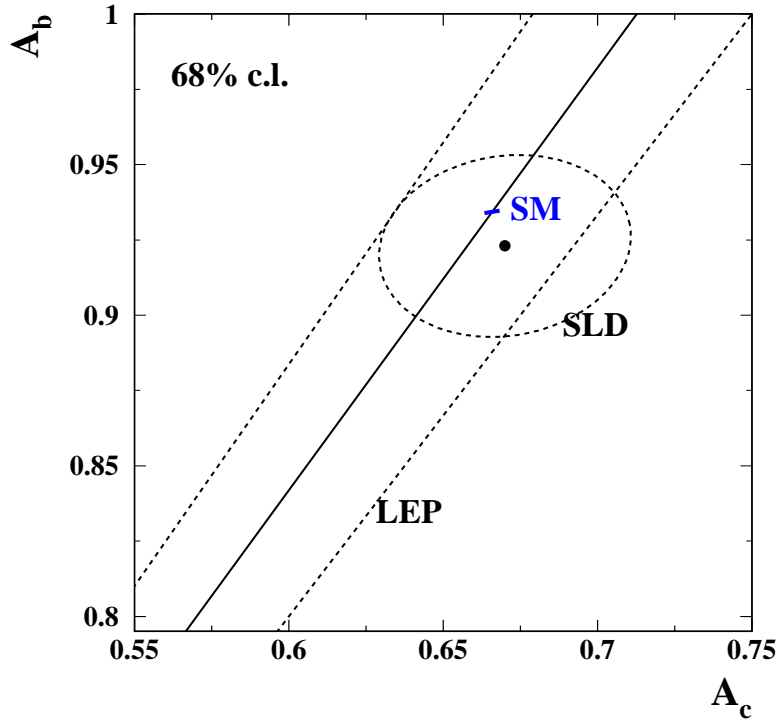
Figure 5.17: Contours in the \mathcal{A}_c - \mathcal{A}_b plane and ratios of forward-backward asymmetries from the SLD and LEP, corresponding to 68 % confidence levels assuming Gaussian systematic errors. The SM prediction for m_t = 178.0 \pm 4.3 GeV, m_H = 300_{-186}^{+700} GeV and \Delta\alpha_{\text{had}}^{(5)}(m_Z^2) = 0.02758 \pm 0.00035 is also shown.
