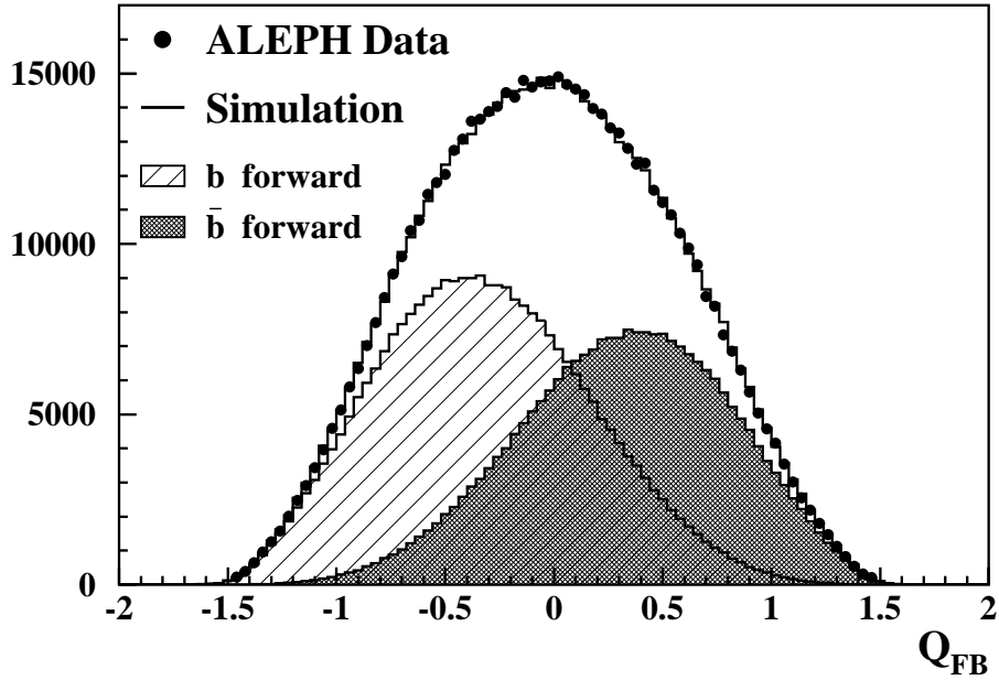
Figure 5.12: Charge separation of the ALEPH neural net tag using jet charge, vertex charge and charged kaons [142]. The asymmetry reflects A_{\text{FB}}^{\text{b}\bar{\text{b}}} diluted by the non-perfect charge tagging.
