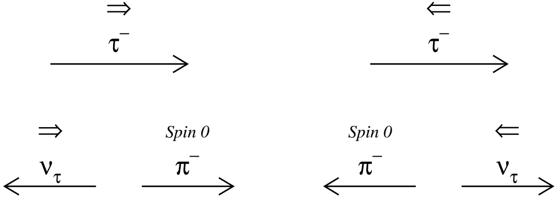
Figure 4.1: Decay configurations for two \tau helicity states for the decay \tau^- \rightarrow \pi^- \nu_\tau . The positive helicity configuration is on the left and the negative configuration is on the right. For each particle, the long arrow depicts the momentum direction while the short double arrow that of the spin. The lower pair of figures is depicted in the helicity rest frame of the parent \tau .
