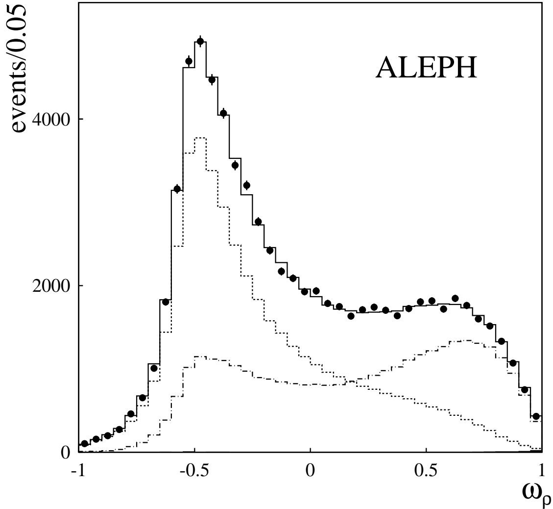
Figure 4.4: The measured spectrum of the polarisation-sensitive variable \omega_\rho , described in the text, for the \tau \rightarrow \rho\nu decays in the ALEPH experiment. The dashed and dashed-dotted lines correspond to the contributions of negative and positive helicity \tau 's, respectively. The small shaded area near \omega=1 is the non- \tau background contribution.
