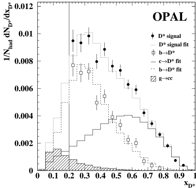
Figure 5.6: D^{*\pm} momentum spectrum for all events and for b\bar{b} and c\bar{c} events from OPAL normalised to the beam energy after subtraction of combinatorial background [130].
