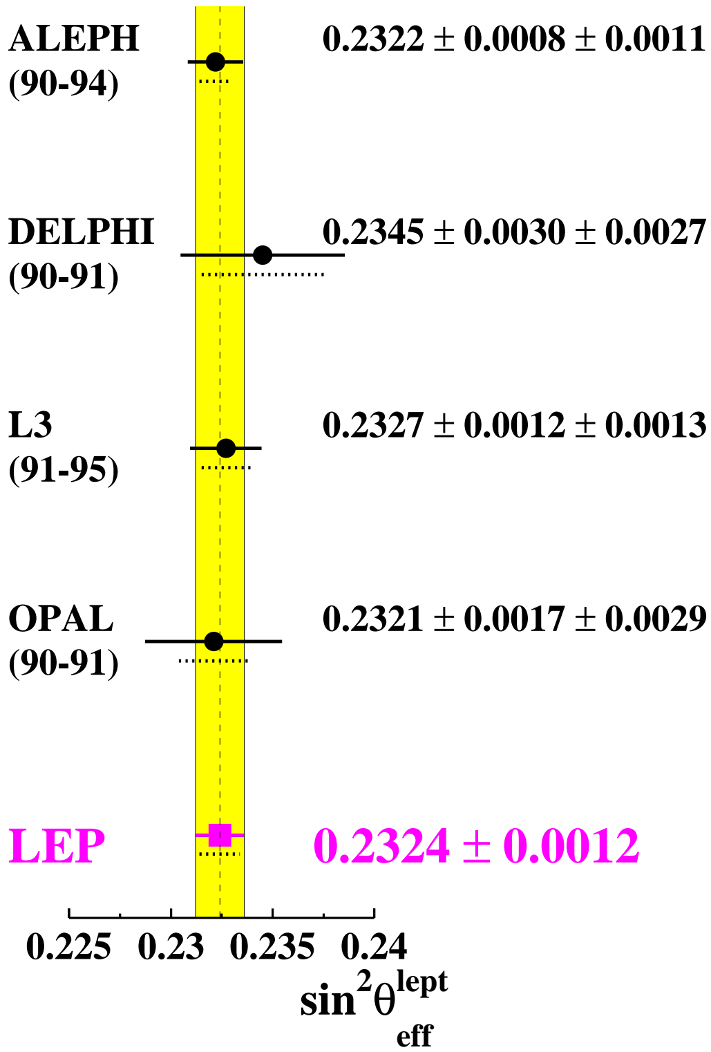
Figure 6.2: The input values and derived average of \sin^2 \theta_{\text{eff}}^{\text{lept}} from Q_{\text{FB}}^{\text{had}} measurements. The total uncertainties are indicated by the solid lines, and the systematic contribution to the uncertainties by the dotted lines.
