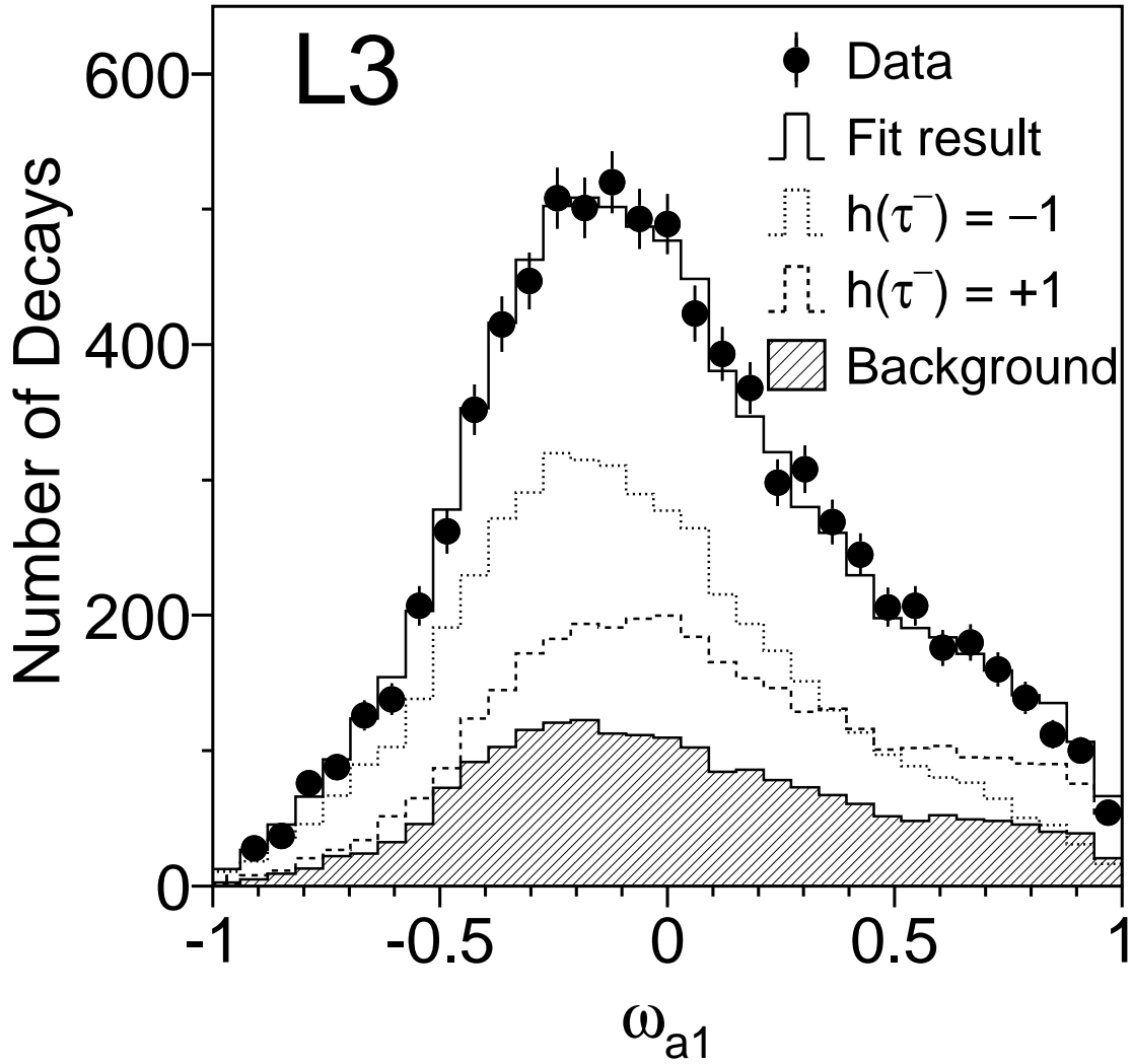
Figure 4.5: The measured spectrum of the polarisation-sensitive variable \omega_{a_1} , described in the text, for the \tau \rightarrow a_1 \nu decays in the L3 experiment. The distributions for both a_1^- \rightarrow \pi^- \pi^+ \pi^- and a_1^- \rightarrow \pi^- \pi^0 \pi^0 decays are combined in this figure. The two helicity components and the background are shown separately.
