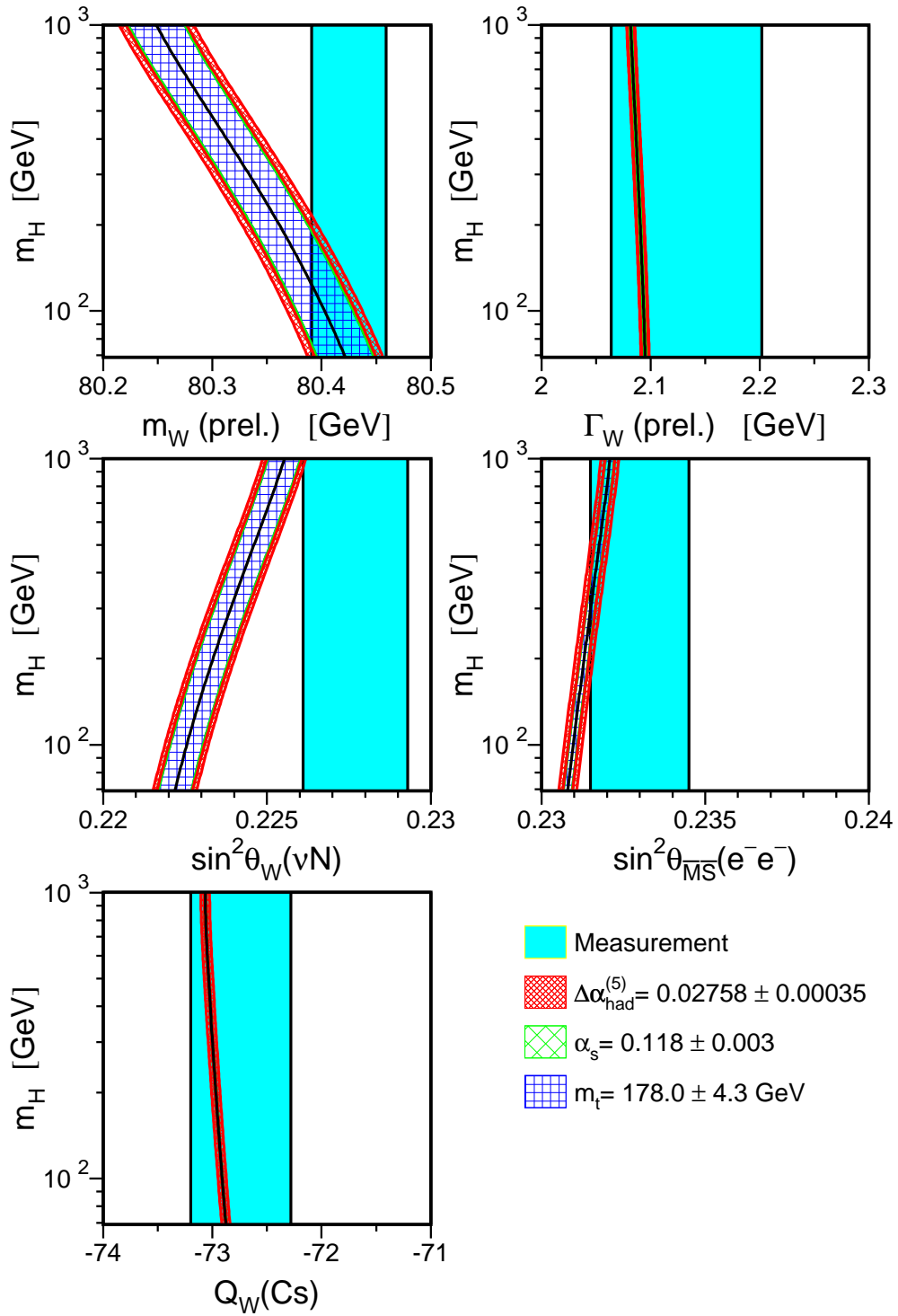
Figure 8.7: Comparison of the combined measurements of m_W and \Gamma_W , and the results from low Q^2 processes \sin^2 \theta_W(\nu N) , \sin^2 \theta_{\overline{\text{MS}}}(m_Z)(e^-e^-) and Q_W (APV) with the SM prediction as a function of the mass of the Higgs boson. The measurement with its uncertainty is shown as the vertical band. The width of the SM band arises due to the uncertainties in \Delta\alpha_{\text{had}}^{(5)}(m_Z^2) , \alpha_s(m_Z^2) and m_t in the ranges indicated. The total width of the band is the linear sum of these uncertainties. The direct measurements of m_W and \Gamma_W used here are preliminary.
