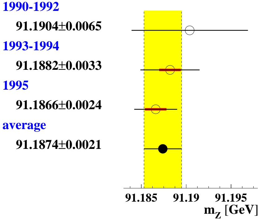
Figure 2.10: m_Z in GeV for three different periods of data taking, before 1993, 1993–1994 and 1995. The second, smaller error bar represents the correlated error component of 1.2 MeV between m_Z^{93-94} and m_Z^{95} . The value of m_Z^{90-92} is essentially uncorrelated with the other two.
