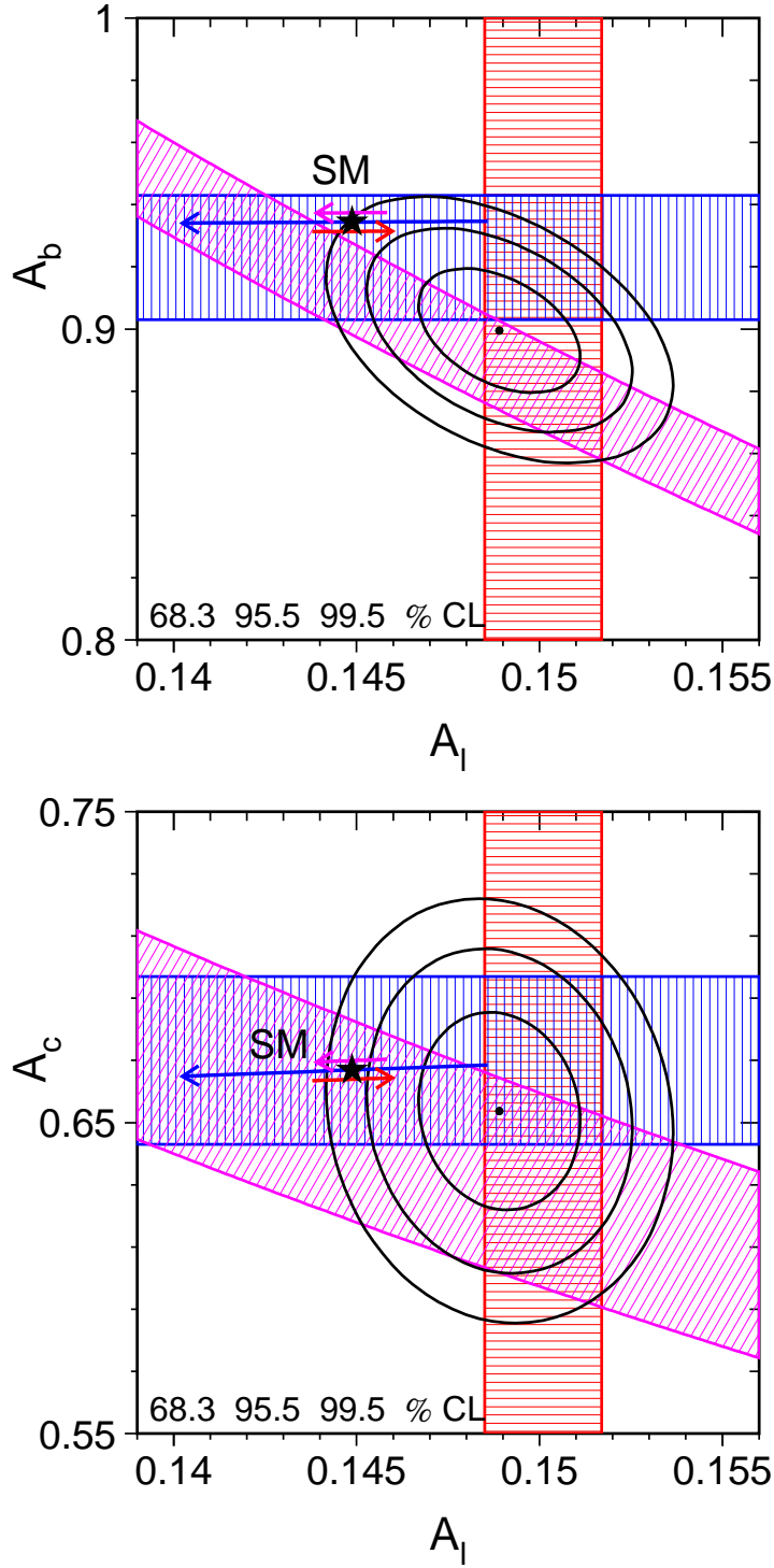
Figure 7.2: Comparison of the measurements of \mathcal{A}_\ell , \mathcal{A}_q and A_{\text{FB}}^{0,q} for (top) b-quarks, and (bottom) c-quarks, assuming lepton universality. Bands of \pm 1 standard deviation width in the (\mathcal{A}_\ell, \mathcal{A}_q) plane are shown for the measurements of \mathcal{A}_\ell (vertical band), \mathcal{A}_q (horizontal band), and A_{\text{FB}}^{0,q} = (3/4)\mathcal{A}_e\mathcal{A}_q (diagonal band). Also shown are the 68%, 95% and 99.5% confidence level contours for the two asymmetry parameters resulting from the joint analysis (Table 7.6). The arrows pointing to the right and to the left show the variation in the SM prediction for varying \Delta\alpha_{\text{had}}^{(5)}(m_Z^2) in the range 0.02758 \pm 0.00035 (arrow displaced vertically upwards), m_H in the range of 300_{-186}^{+700} GeV, and m_t in the range 178.0 \pm 4.3 GeV (arrow displaced vertically downwards). All arrows point in the direction of increasing values of these parameters.
