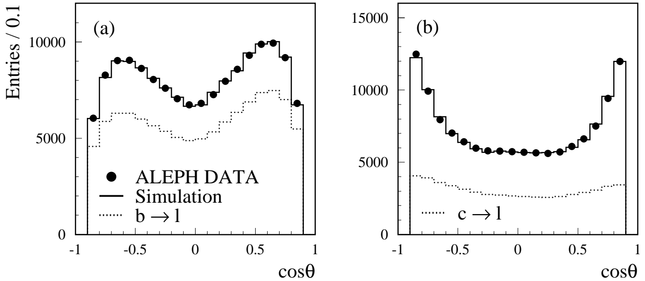
Figure 5.10: Reconstructed \cos\theta distribution from the ALEPH asymmetry measurements with leptons for a) the b-enriched and b) the c-enriched sample [141]. The full histogram shows the expected raw angular distribution in the simulation. The dashed histogram show the signal component.
