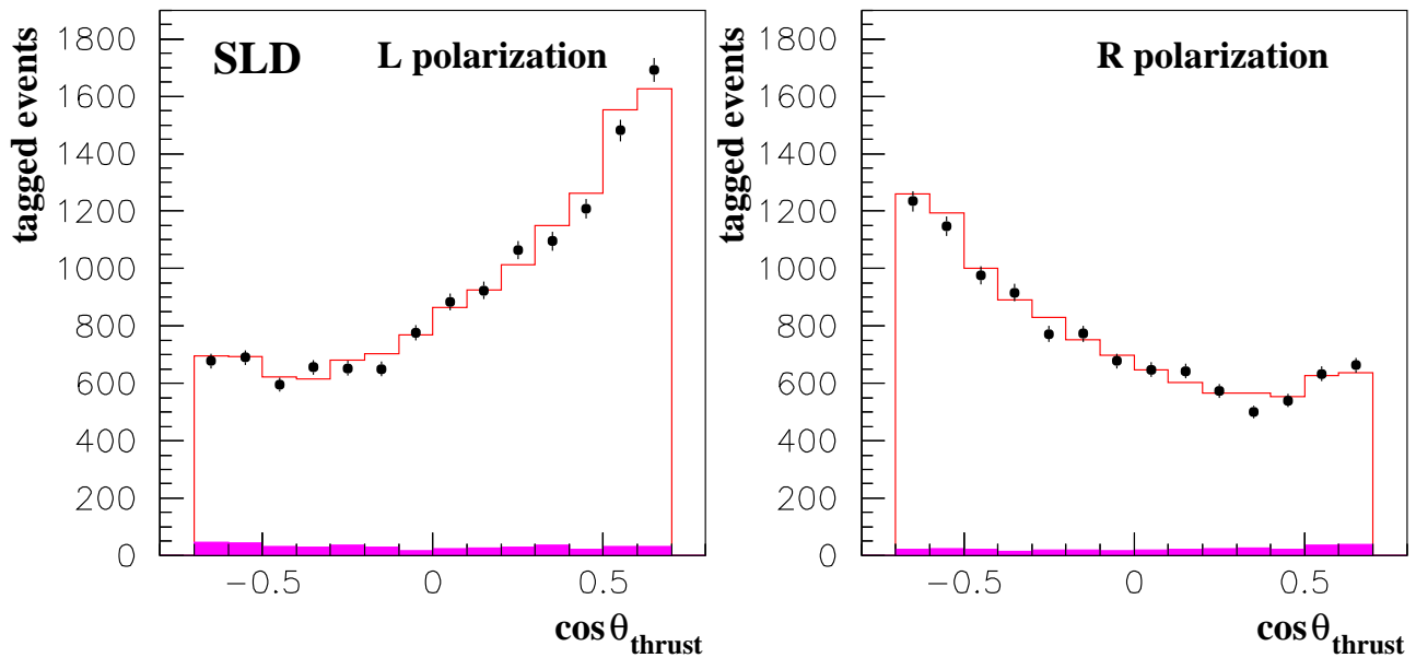
Figure 5.11: Reconstructed \cos\theta distributions from the SLD vertex charge \mathcal{A}_b analysis for events with left-handed and right-handed electron beam polarisations. The shaded region corresponds to u\bar{d}c background in the sample estimated from Monte Carlo.
