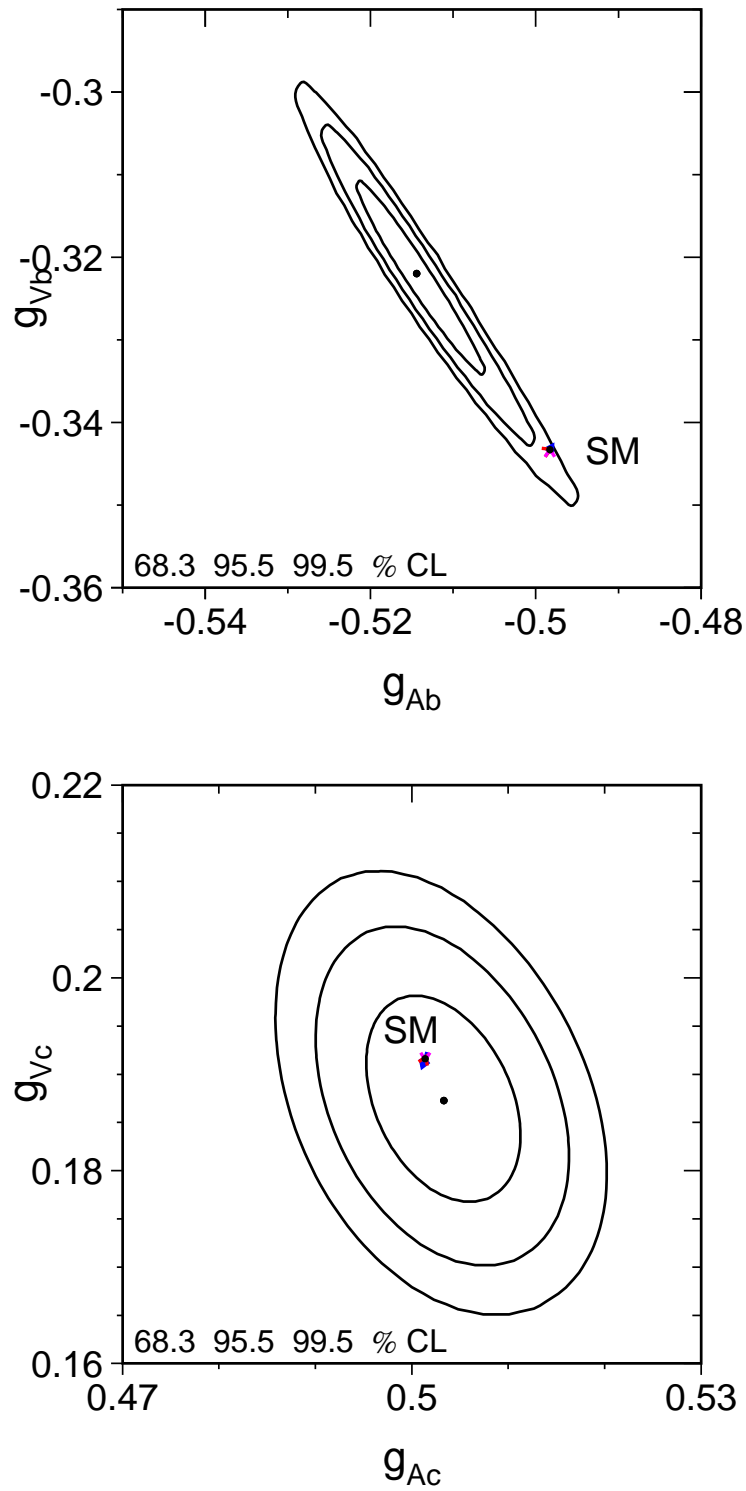
Figure 7.4: Comparison of the effective vector and axial-vector coupling constants for heavy quarks, using results on leptons and assuming lepton universality (Table 7.9). Top: b quarks; bottom: c quarks. Compared to the experimental uncertainties, the SM predictions for the heavy quarks b and c have negligible dependence on the SM input parameters.
