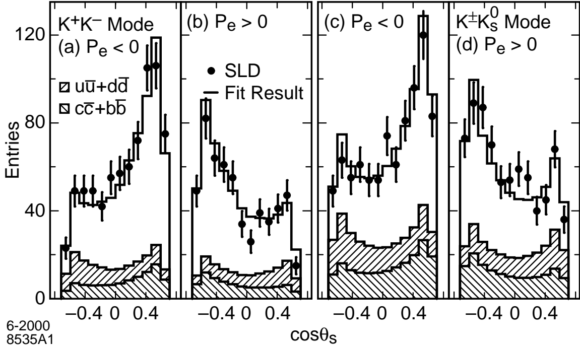
Figure F.2: Measured s-quark polar angle distributions (dots) for selected SLD events in the (a),(b) K^+K^- and (c),(d) K^\pm K_S^0 modes, produced with (a),(c) left- and (b),(d) right-polarised electron beams. The histograms represent the result of a simultaneous fit to the four distributions, and the upper (lower) hatched areas indicate the estimated u\bar{u}+d\bar{d} ( c\bar{c}+b\bar{b} ) backgrounds.
