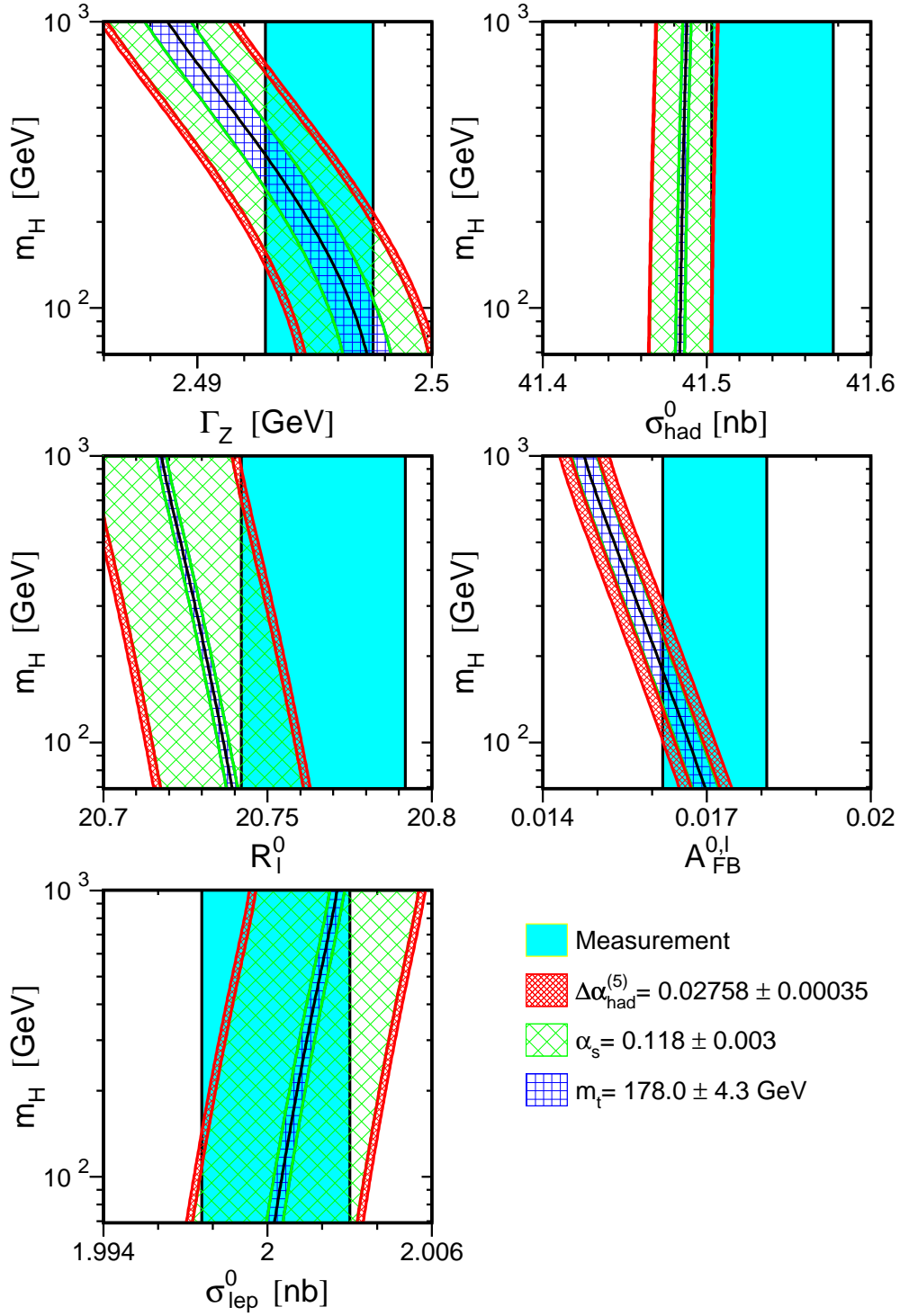
Figure 8.4: Comparison of the LEP combined measurements of \Gamma_Z , \sigma_{\text{had}}^0 , R_\ell^0 , A_{\text{FB}}^{0,\ell} and \sigma_{\text{lep}}^0 with the SM prediction as a function of the mass of the Higgs boson. The measurement with its uncertainty is shown as the vertical band. The width of the SM band arises due to the uncertainties in \Delta\alpha_{\text{had}}^{(5)}(m_Z^2) , \alpha_s(m_Z^2) and m_t in the ranges indicated. The total width of the band is the linear sum of these uncertainties.
