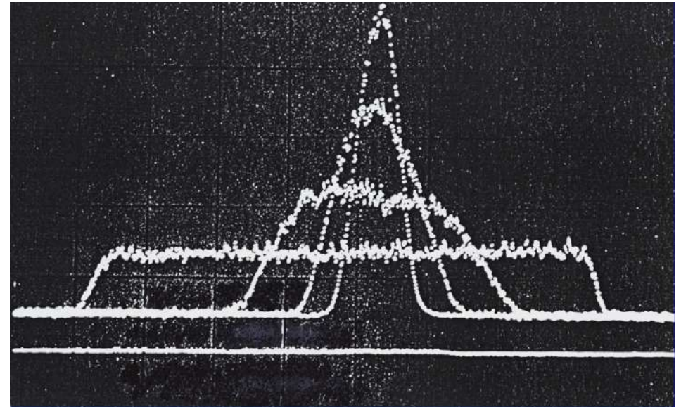
Schottky scan after 1, 2 and 4 minutes .
