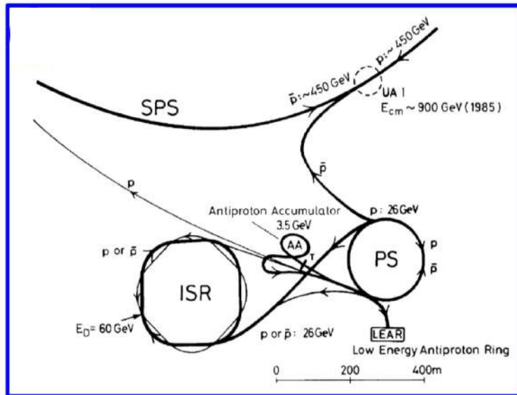
CERN p\bar{p} complex in the '80s
