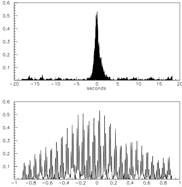
Fig. 1: The NAUTILUS response to the CR shower with particle density 2812 \text{ par./m}^2 , filtered energy (K) versus time (s), centered at the CR shower arrival time. The lower figure is a zoom of the upper one. We note the oscillation related to the beating of the two resonant modes and the decay due to the detector bandwidth, \delta f \sim 0.4 \text{ Hz} .
