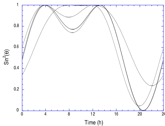
Fig. 1. Amplitude response \sin^2\theta(t) of the five IGEC detectors versus Universal Time for signals incoming from the Galactic Center during one day.
