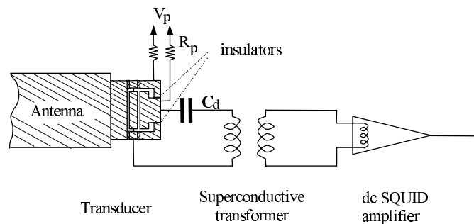
Figure 2. Read-out scheme.
