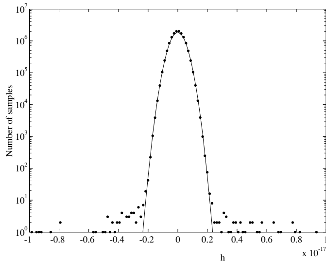
Figure 5. Distribution of 24 h of EXPLORER data—day 161 of 2001.
