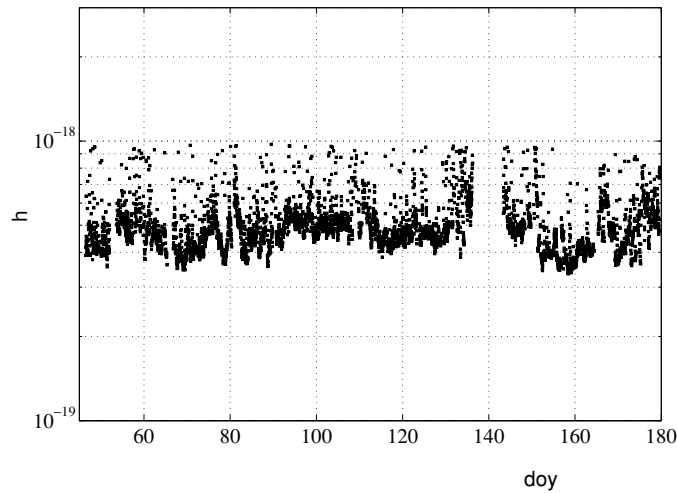
Figure 4. Operation from January to June 2001—30 min averaged data.
