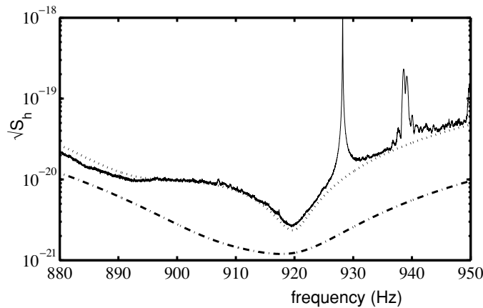
Figure 3. \sqrt{S_h} over 10 h of data.
