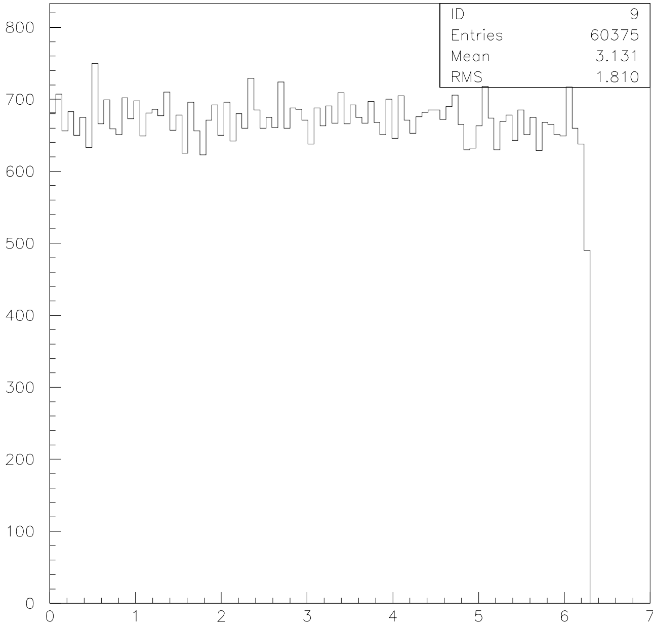
DISTR. FI COMPTON
