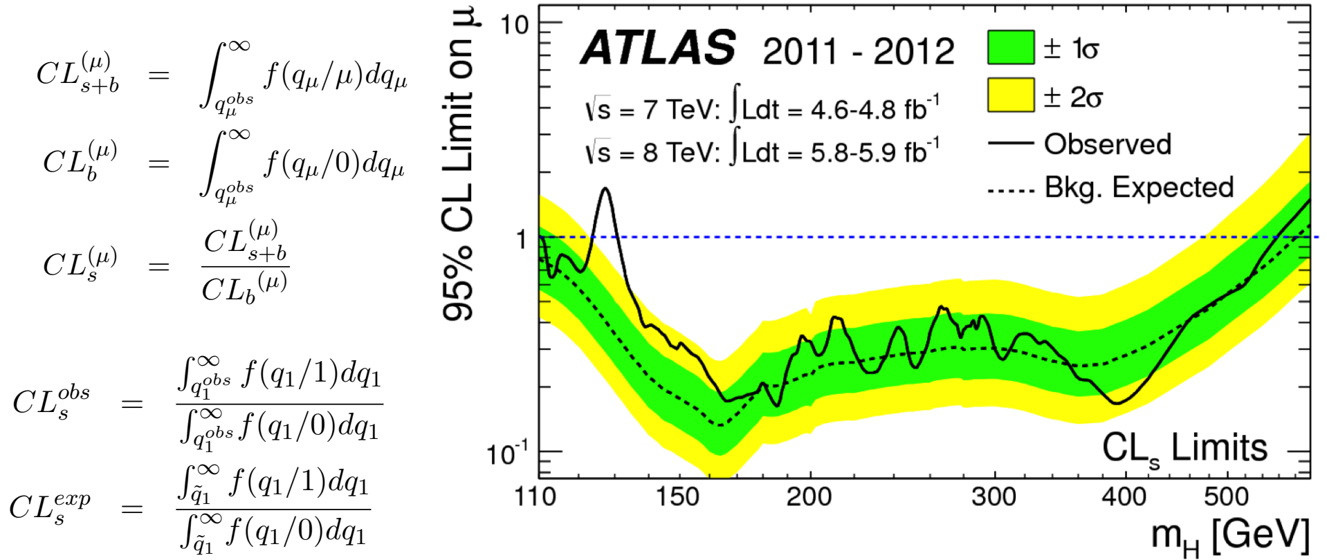
FIGURE 28. Exclusion "Brazilian plot". Observed (solid) and expected(dashed) 95% CL upper limits on the signal strength \mu as a function of M_H . \pm 1 (green) and \pm 2 (yellow) std.deviation bands are also shown for the expected limit. (taken from ATLAS collaboration, Phys.Lett. B716 (2012) 1-29)
