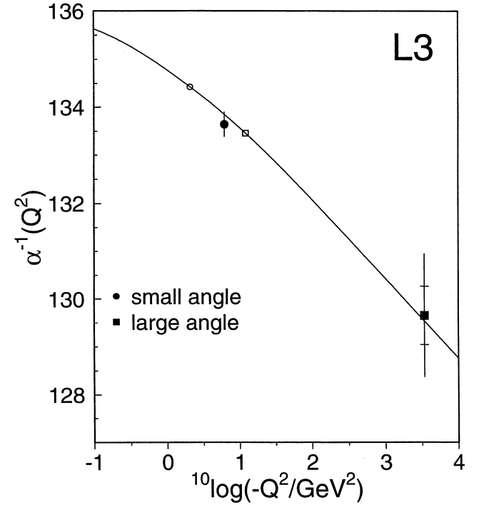
Fig. 3. Measurements of \alpha^{-1}(Q^2) for Q^2 < 0 . The results of the small-angle and large-angle Bhabha scattering measurements described in this article are shown as a solid circle and square, respectively. The corresponding reference Q^2 values at which the value of \alpha^{-1}(Q^2) is fixed to its expectation are shown as open symbols. The error bar on the large-angle point indicates the experimental and the total uncertainty.
