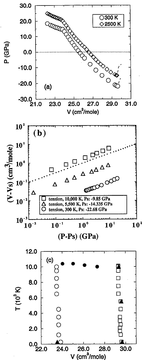
FIG. 3. SiO 2 cristobalite under compression and tension (a) P - V relations; the 2500 K curve has been displaced upward 5 GPa for clarity. (b) Log-log plots of V - V_s against P - P_s showing linearization with mean-field exponent 0.5 (dotted line). (c) Limiting volumes under compression and tension plotted against volume [note distinction from Fig. 1(c) to emphasize isochoric limits to metastability under compression (open squares), and tension (open circles)]. Filled circles denote nucleated melting points, and filled triangles denote V_s obtained from power-law fits of part (b). In the case of the simulated "cristobalite," the collapse at 300 K occurs 25% below the pressure of the laboratory phenomenon (22 GPa [8]): our potential function is too approximate for accurate predictions on SiO 2 .
