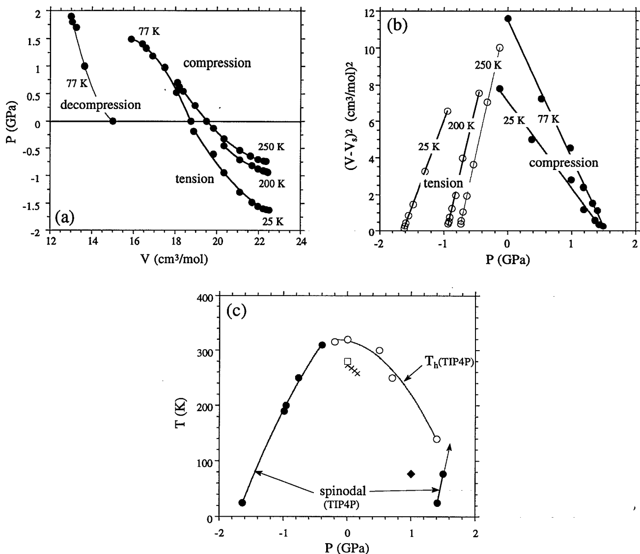
FIG. 1. Ice I_h under compression and tension. (a) P - V relations at several temperatures. Solid lines give the reversible behavior. (b) Tests of mean-field behavior of volume near compression and tension stability limits ( P_s, T_s ). (c) Values of P_s that linearize the plots in part (b) and define the stability limits under compression (filled circles). Open circles denote the nucleated fusion points (non-spinodal). The open square is the equilibrium melting point at atmospheric pressure, and crosses show the melting line. The diamond shows the laboratory amorphization pressure at 80 K [4].
