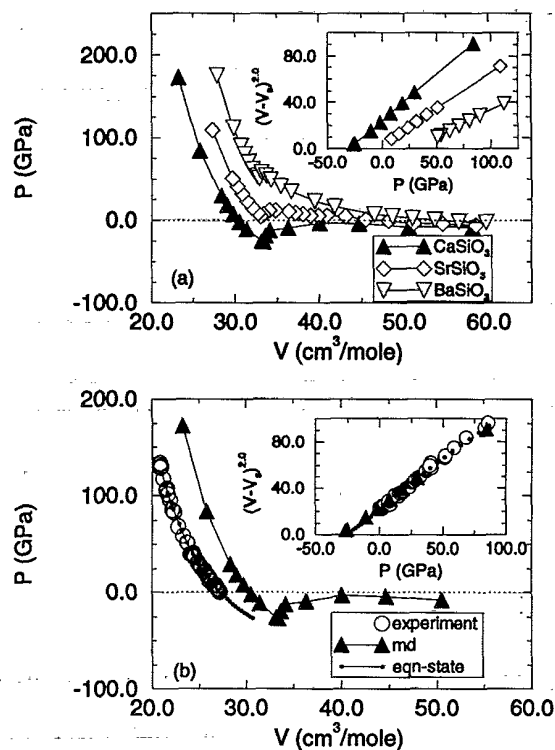
FIG. 4. (a) Variation of pressure with volume during decompression of simulated alkaline earth metasilicate perovskites M[\text{II}]\text{SiO}_3 . Note how a change of cation size parameter shifts the spinodal limit on perovskite stability from positive to negative pressures without changing the limiting volume. The inset shows how data over a wide volume range are consistent with the existence of a spinodal limit slightly beyond the observed rupture point (for \text{CaSiO}_3 , P_s = -30.8 \text{ GPa} , V_s = 35.3 \text{ cm}^3 ; \text{SrSiO}_3 , P_s = -6.1 \text{ GPa} , V_s = 35.7 \text{ cm}^3 ; \text{BaSiO}_3 , P_s = 48.6 \text{ GPa} , V_s = 36.1 \text{ cm}^3 ). (b) Variation of pressure with volume for laboratory and simulated \text{CaSiO}_3 . The limitation of the rigid ion potential as parametrized by us is manifested by a discrepancy in the pressure. However, the curvatures are comparable since the quadratic plots testing the mean field stability limit [inset of (b)] superimpose. Quantitative agreement is obtainable with modified potentials based on those of Matsui for \text{MgSiO}_3 (see [18]).
