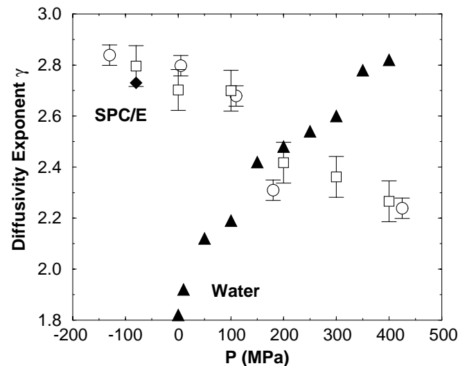
FIG. 3. Pressure dependence of the diffusivity exponent \gamma defined by D \sim (T/T_c - 1)^\gamma . The symbols may be identified as follows: ( \circ ) \gamma calculated from simulation along isochores; ( \square ) \gamma calculated from simulation along isobars, which are estimated by interpolation of the isochoric data for D ; ( \diamond ) \gamma calculated in Ref. [11] along the -80 \text{ MPa} isobar; ( \blacktriangle ) experimental measurements of \gamma in water from Ref. [3]. Note that the SPC/E potential fails to reproduce the experimentally observed behavior of \gamma under pressure.
