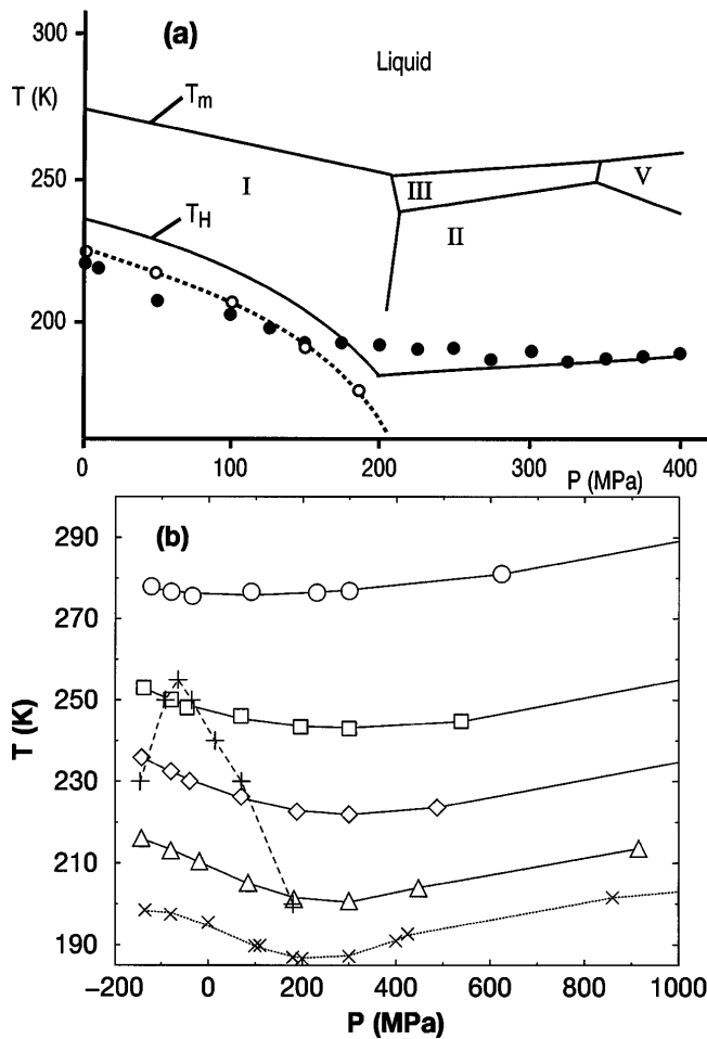
FIG. 1. (a) Phase diagram of water, showing the extrapolated divergence of the isothermal compressibility ( \circ ) [2] and the extrapolated divergence of D ( \bullet ) [3]. The different locations of these divergences suggest that the phenomena may arise from different explanations. Also shown are the melting line ( T_m ) and coexistence lines of several ice polymorphs and the experimental limit of supercooling ( T_H ). (b) Isochrones of D from simulation. The lines may be identified as follows: D = 10^{-5} \text{ cm}^2/\text{s} ( \circ ); D = 10^{-5.5} \text{ cm}^2/\text{s} ( \square ); D = 10^{-6} \text{ cm}^2/\text{s} ( \diamond ); D = 10^{-7} \text{ cm}^2/\text{s} ( \triangle ). The diffusion is also fit to D \sim (T/T_c - 1)^\gamma . The locus of T_c is indicated by ( \times ). For reference, the ( + ) symbols indicate the locus of T_{MD} found in Ref. [20].
