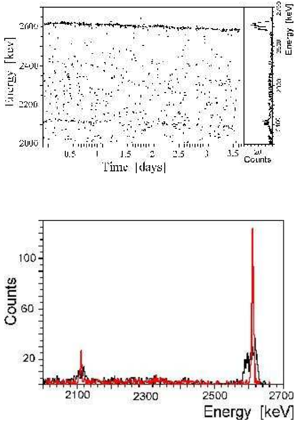
Figure 32: Effects of the system thermal instabilities on the worsening of the detector energy resolution (above). Comparison between calibration spectra before (black curve: \Delta E_{2615}^{FWHM} = 30 keV) and after (red curve: \Delta E_{2615}^{FWHM} = 6 keV) the stabilization procedure.
