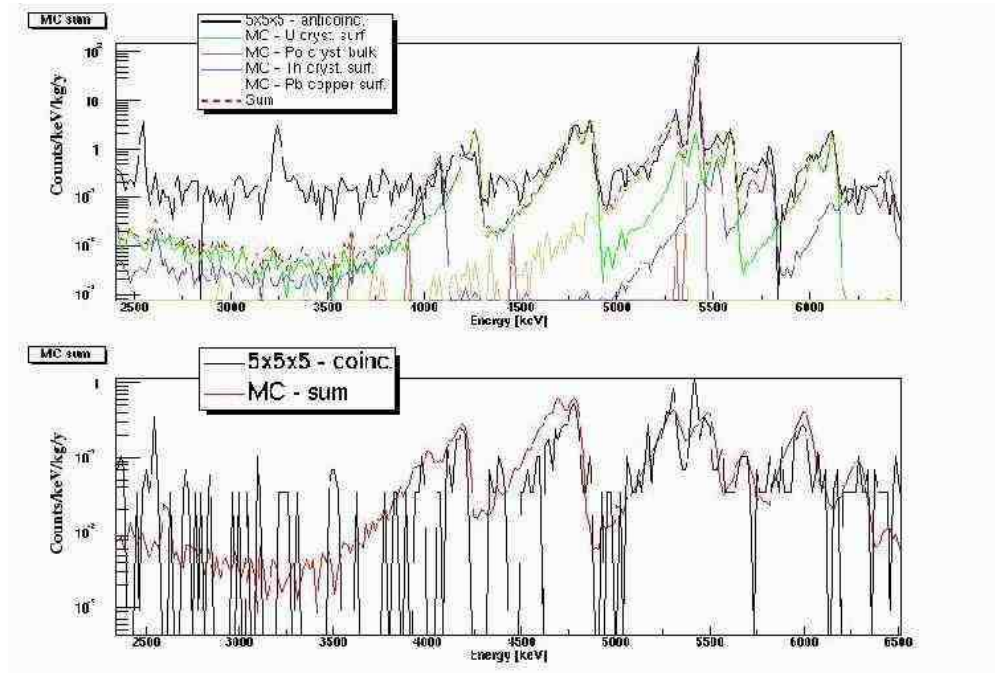
Figure 29: Comparison between Monte Carlo and CUORICINO anticoincidence (top) and coincidence (bottom) spectra in the case of the \text{TeO}_2 crystal surface contaminations ( \lambda \sim 1 \mu\text{m} ) specified in the figure.
