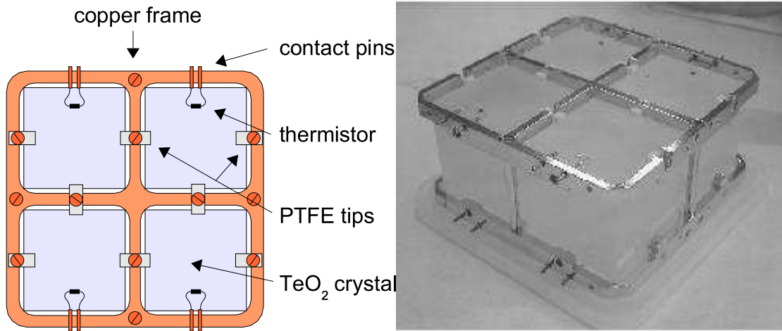
Figure 36: A four detector module.
