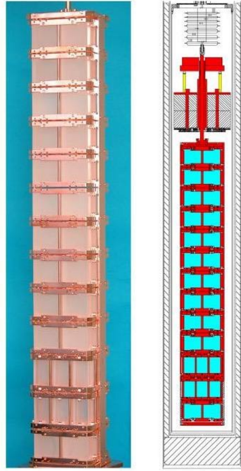
FIG. 1 (color online). Scheme of CUORICINO.
