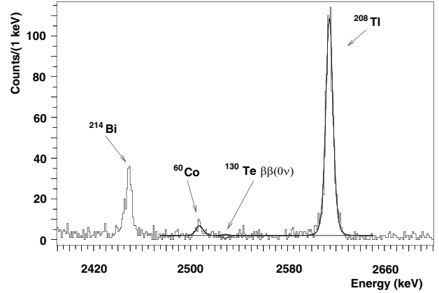
FIG. 2. Anticoincidence spectrum of the sum of the two electron energies in the region of neutrinoless 0\nu\beta\beta decay.
