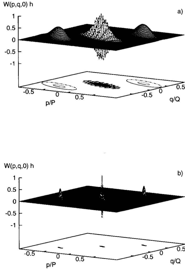
Figure 1. Wigner function at time 0 corresponding to the cat state (16) for k_B T / \hbar \gamma = 100 . In case a) we have P = 20\sqrt{\hbar m \gamma} and Q = 2\sqrt{m \gamma / \hbar} while in b) P = 100\sqrt{\hbar m \gamma} and Q = 10\sqrt{m \gamma / \hbar} .
