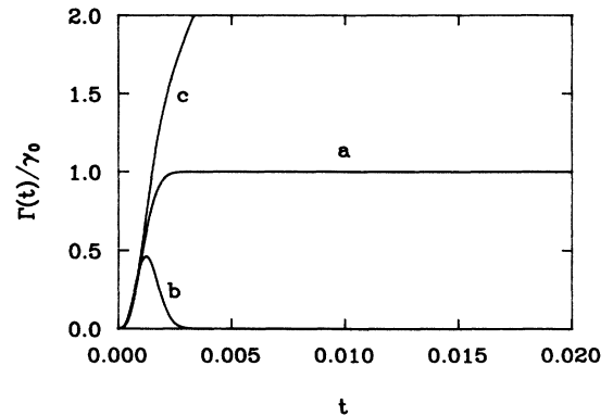
FIG. 1. The dissipative coefficient for the a ohmic ( n=1 ), b supraohmic ( n=3 ), and c subohmic ( n=\frac{1}{2} ) environments. The parameters are measured in units of the renormalized frequency \Omega , which is set to unity [see Eq. (2.45)]. We consider the cases \gamma_0=0.3 , \Lambda=2000 .
