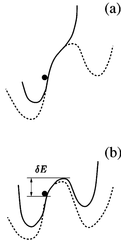
FIG. 2. Schematic sketch of the pitfalls associated with the straight path approximation, on calculating the energy profile. Lower (upper) sketch shows the case when the location of the instantaneous configuration is close to (far from) a saddle point. The net effect of the straight path approximation is an artificial rise of the potential energy profile with negative curvature.
