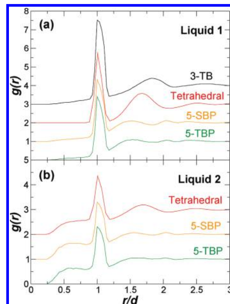
Figure 4. Radial distribution function g(r) as a function of scaled distance r/d , where d is the typical bonding distance. For visual clarity, g(r) for 5-SBP, tetrahedral, and 3-TB are shifted vertically by 1, 2, and 3, respectively. (a) g(r) of the first liquid, including geometries 3-TB ( T=0.08 , \rho d^3=0.28 ), tetrahedral ( T=0.073 , \rho d^3=0.64 ), 5-SBP ( T=0.0826 , \rho d^3=0.86 ), and 5-TBP ( T=0.0825 , \rho d^3=0.82 ). (b) g(r) of the second liquid, including tetrahedral ( T=0.073 , \rho d^3=1.29 ), 5-SBP ( T=0.0826 , \rho d^3=1.43 ), and 5-TBP ( T=0.0825 , \rho d^3=1.44 ).
