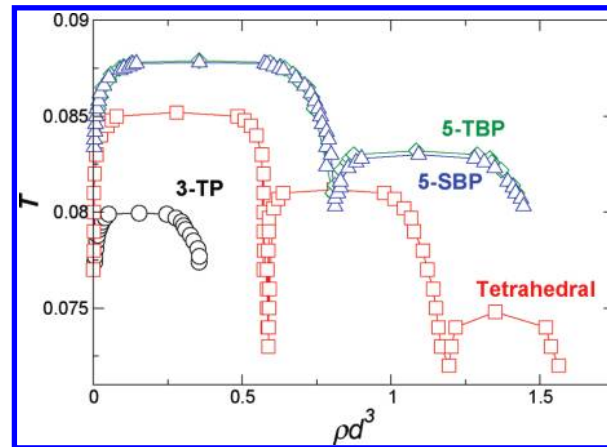
Figure 2. T - \rho phase diagram of geometries 3-TP, tetrahedral, 5-TBP, and 5-SBP. The density is scaled by the cube of the bonding distance d^3 such that the density is comparable to the density of hard-sphere systems.
