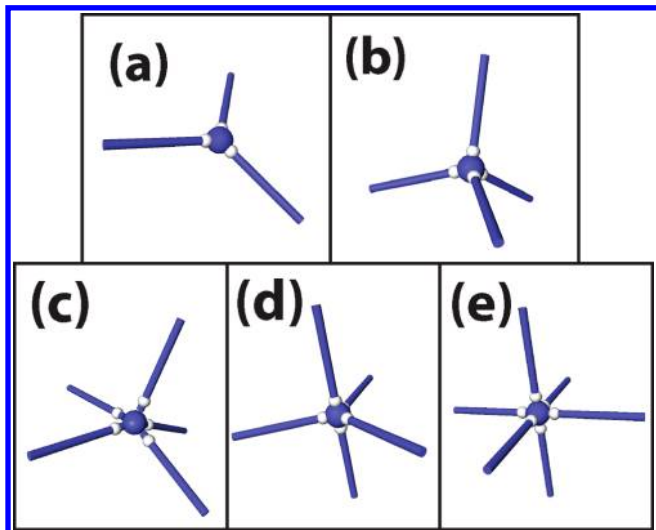
Figure 1. Cartoon of the geometries of the DNA-functionalized nanoparticles studied: (a) triangular planar (3-TP), (b) tetrahedral, (c) square-based pyramid (5-SBP), (d) triangle-based bipyramid (5-TBP), (e) octahedral. The central sphere indicates the NP, while the cylinder represents the sequence of DNA base pairs tethered to the central core at the small sphere locations.
