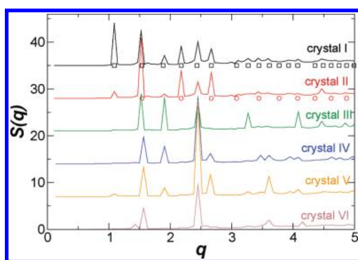
Figure 11. S(q) for octahedral geometry. For clarity, lines are shifted vertically so that each crystal is 7 units apart. The black squares below crystal I are the theoretically expected locations for the peaks of a perfect simple cubic lattice; similarly, the red circles below crystal II are the expected locations for the peaks of a perfect BCC lattice.
