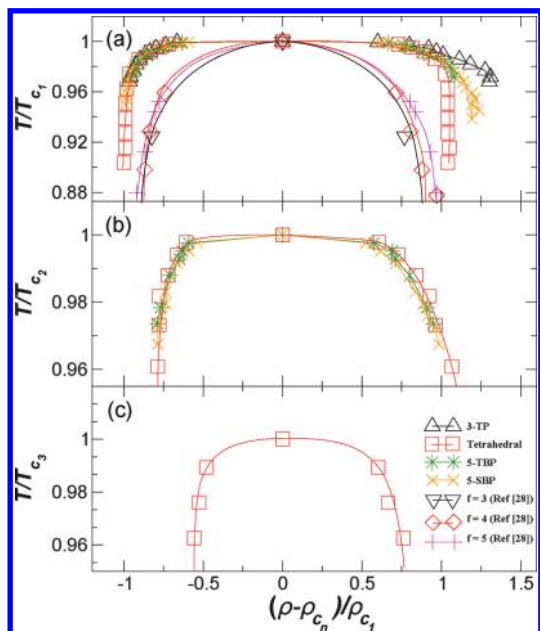
Figure 3. T - \rho phase diagram with density shifted by respective critical densities and scaled by first critical density; the temperature is scaled by the respective T_c . The solid lines are guides to the eye. (a) The first phase transition, analogous to a gas-liquid transition, for geometries 3-TP, tetrahedral, 5-TBP, and 5-SBP. In addition, we show results from patchy colloids from reference with either 3, 4, or 5 patches. 28 (b) The second phase transition, a liquid-liquid phase transition, for geometries 5-TBP, 5-SBP, and tetrahedral. (c) The third phase transition for tetrahedral geometry.
