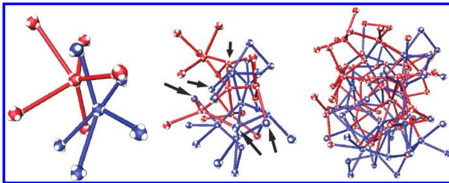
Figure 6. Visualization of the two interpenetrating networks up to chemical distance D = 1 , D = 2 , and D = 3 for 5-SBP at T = 0.0826 , \rho d^3 = 1.44 . We assign two different colors to illustrate the two distinct interpenetrating networks. The arrows indicate locations where the two networks intersect each other as a result of distortion.
