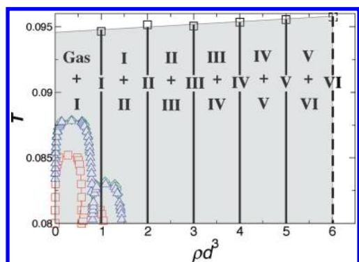
Figure 10. T - \rho phase diagram of multiple crystals formed by octahedral nanoparticles. The density is scaled by d^3 . The gray regions indicate phase coexistence between crystals, except for the smallest density, where crystal I coexists with the gas phase. Crystal VI is observed, but we are not able to obtain a reliable melting temperature, and therefore represented by the dashed lines. For comparison, we also show phase boundaries of the amorphous systems obtained in Figure 2: red squares are for the tetrahedral orientation; blue triangles are for the 5-SBP; green diamonds are for the 5-TBP.
