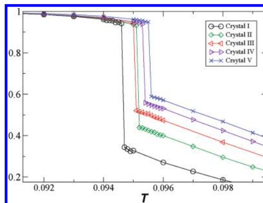
Figure 9. Percentage of intact bonds as a function of T on heating for crystals I–V. The discontinuity provides an upper limit on the melting temperature.
