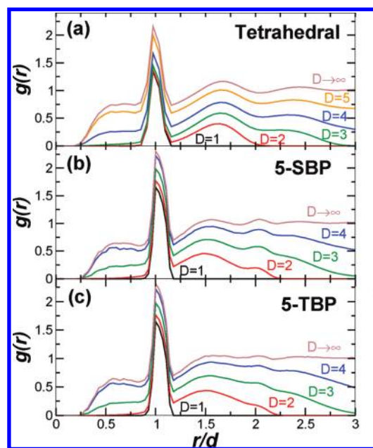
Figure 5. g(r) restricted to bonded neighbors up to a specific chemical distance D for the second liquid of (a) tetrahedral geometry ( T=0.073 , \rho d^3=1.29 ), (b) 5-SBP ( T=0.0826 , \rho d^3=1.43 ), and (c) 5-TBP ( T=0.0825 , \rho d^3=1.44 ).
