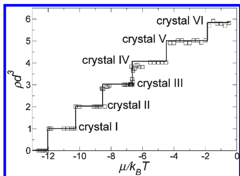
Figure 7. \rho - \mu diagram of six crystals at T = 0.08311 . The density is scaled by d^3 , where d is the typical bonding distance. The line is a guide to the eye.
