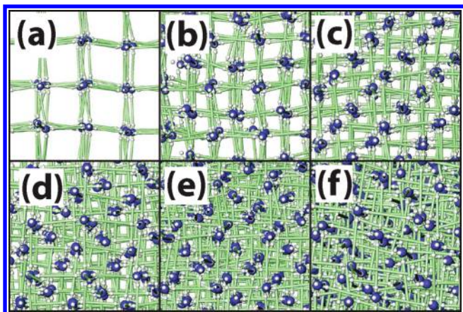
Figure 8. Visualization of the interpenetrating lattices of (a) crystal I ( T = 0.08311 , \rho d^3 = 1.0 ), (b) crystal II ( T = 0.08311 , \rho d^3 = 2.0 ), (c) crystal III ( T = 0.08311 , \rho d^3 = 3.0 ), (d) crystal IV ( T = 0.08311 , \rho d^3 = 4.0 ), (e) crystal V ( T = 0.08311 , \rho d^3 = 5.0 ), and (f) crystal VI ( T = 0.08310 , \rho d^3 = 6.03 ). Specifically, in (b), the core of a DNA complex locates roughly in the center of the other lattice unit cell, a result of two interpenetrating lattices. Because of the large amount of empty space, this motif can be repeated.
