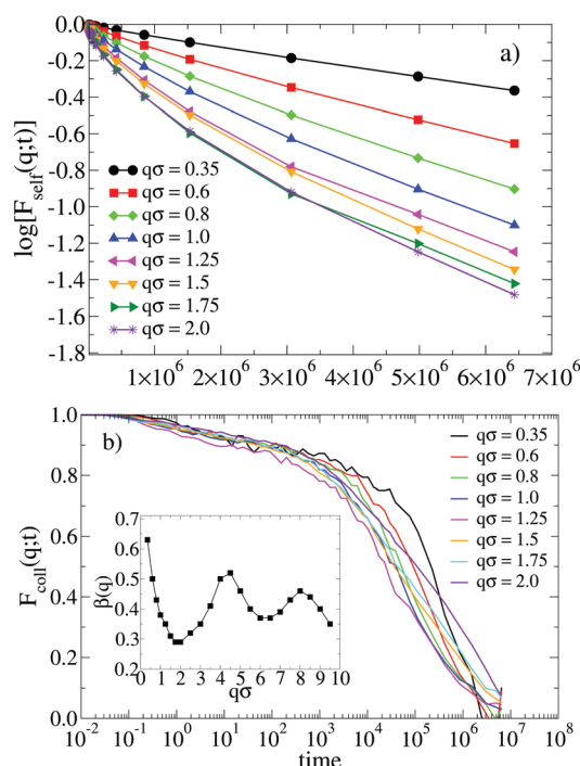
Fig. 17 (a) Linear-linear plot of \log(F_{\text{self}}(q, t)) for q\sigma \in [0.35, 2] at T = 0.1025 (we added solid symbols to highlight the longest correlation times), (b) F_{\text{coll}}(q, t) for q\sigma \in [0.35, 2] at T = 0.1025 . The inset in (b): \beta(q) exponents of the stretched exponential fit (eqn (A.1)) as a function of q .
