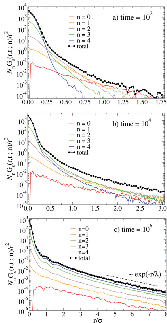
Fig. 7 Partial self van Hove functions \mathcal{N}_n G_s(r, t; n)/r^2 at T = 0.1025 for the different populations of particles according to their initial number of bonds, n \in \{0,1,2,3,4\} . (a) t = 10^2 , (b) t = 10^4 , and (c) t = 10^6 . The figure also shows the corresponding G_s(r, t)/r^2 for the total number of particles (black lines with solid circles). In (c) we also show an exponential decay with \lambda/\sigma = 1.2 (dashed line) which is slightly different from that present in Fig. 6(b) since there is a difference between the longest time in this figure and that corresponding to Fig. 6(b) ( t = 10^6 and t = 6 \times 10^6 respectively).
