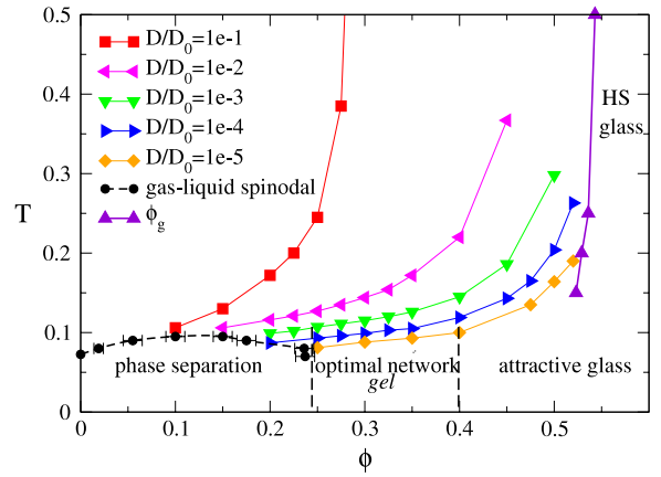
Figure 7. Phase diagram, partially redrawn from [47], with the addition of the iso-diffusivity lines, covering 4 orders of magnitude in D/D_0 , as well as the glass line \phi_g extrapolated from power-law fits.
