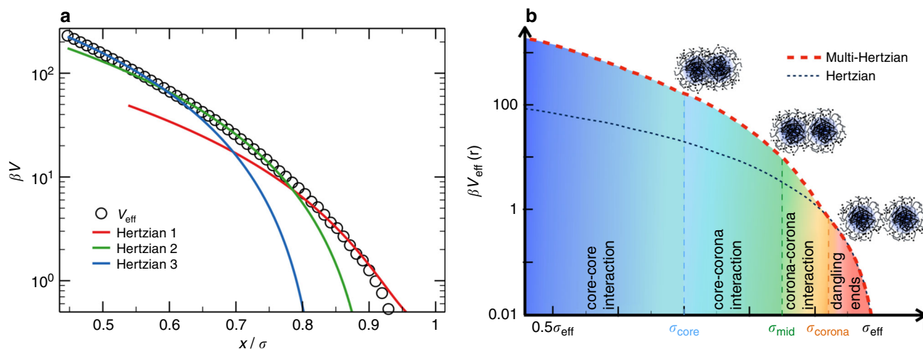
Fig. 5 The multi-Hertzian model. a Calculated effective potential between two microgels as a function of their center-to-center distance. Lines are fits to three different Hertzian contributions, labeled respectively as Hertzian 1, which corresponds to the calculated elastic moduli 40 and whose effective diameter \sigma is used to rescale the x -axis, Hertzian 2 and Hertzian 3 representing the contributions of the inner structure of the microgels. For the reported microgel, the fitted strengths are U_1 = 335k_B T , U_2 = 1182k_B T and U_3 = 2617k_B T and the fitted lengths are \sigma_1 = \sigma , \sigma_2 = 0.92\sigma and \sigma_3 = 0.835\sigma in good qualitative agreement with the ones used to fit experimental data whose parameters are given in Table 2; b the model describing experimental data with the employed interactions lengths: \sigma_{\text{core}} , below which core-core interactions take place, \sigma_{\text{mid}} relevant to the onset of core-corona interactions and \sigma_{\text{corona}} which reflect the heterogeneous nature of the outer corona shell. A comparison with the Hertzian model is also provided. Note the logarithmic scales on the y -axis for both panels
